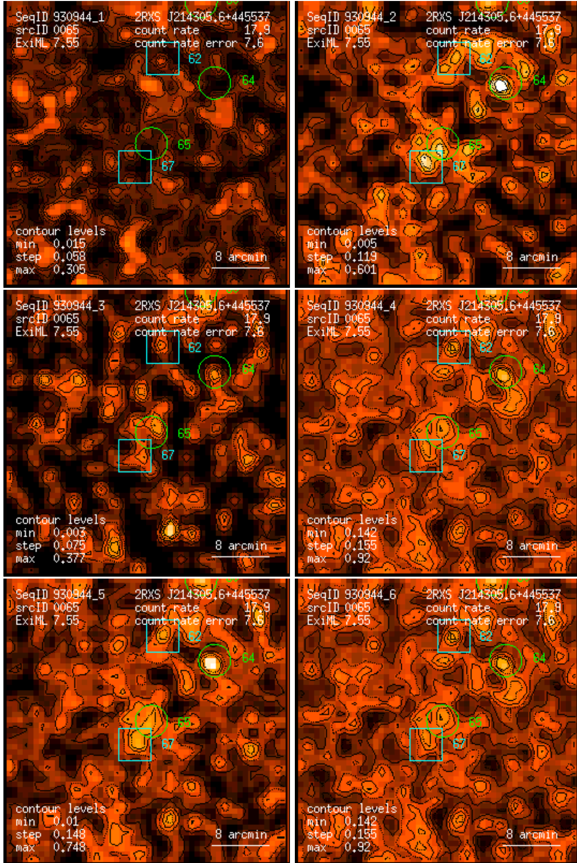
Figure 65: RASS 930944: detection 0065: band rate images, Gaussian filter: (1) PSPC channels 11 – 41, (2) 52 – 90, (3) 91 – 201, (4) 11 – 235, (5) 52 – 201, (6) 11 – 201. Broad band rates in counts/ks. Band rate contour levels in counts/ks/arcmin 2 .
