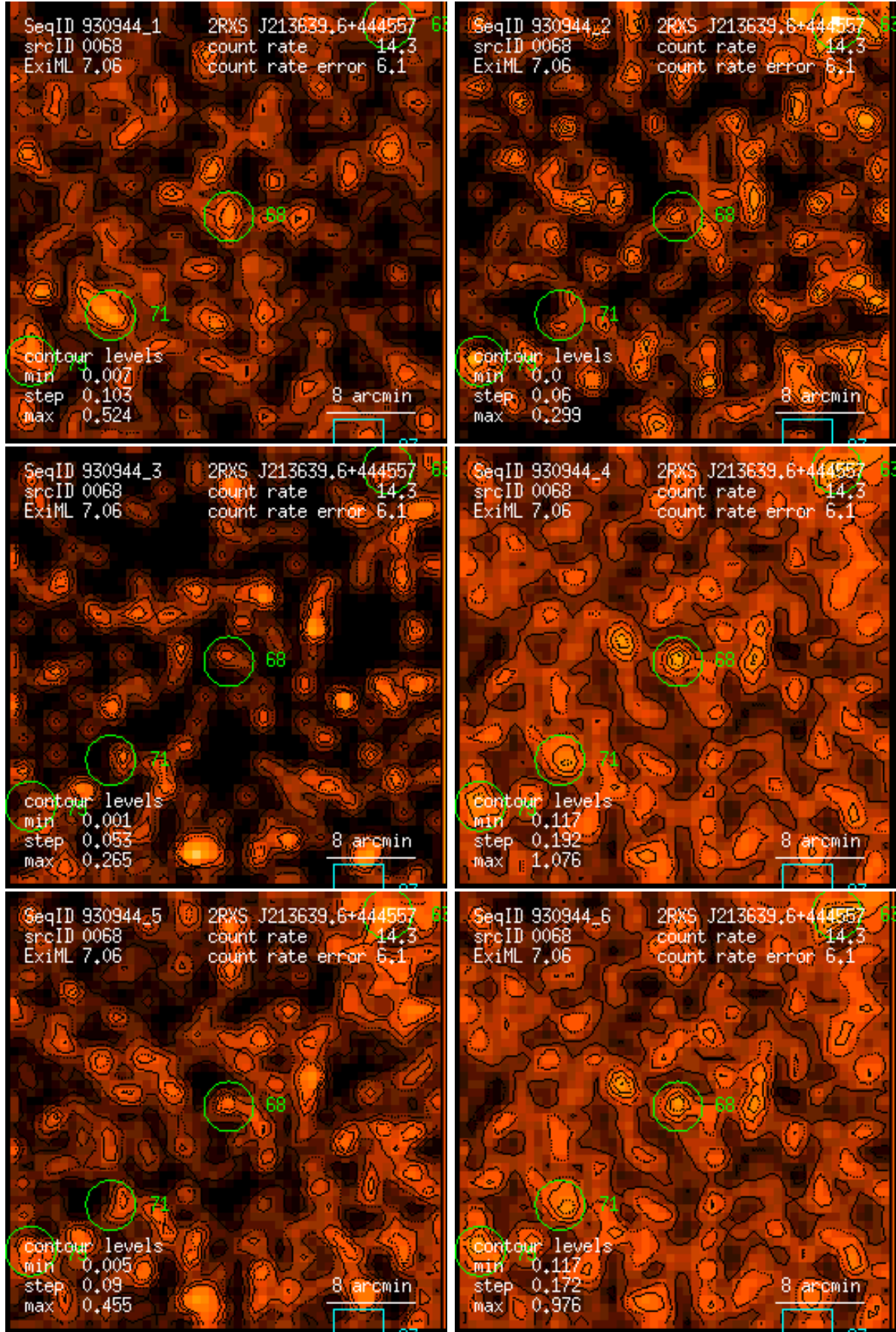
Figure 68: RASS 930944: detection 0068: band rate images, Gaussian filter: (1) PSPC channels 11 – 41, (2) 52 – 90, (3) 91 – 201, (4) 11 – 235, (5) 52 – 201, (6) 11 – 201. Broad band rates in counts/ks. Band rate contour levels in counts/ks/arcmin 2 .
