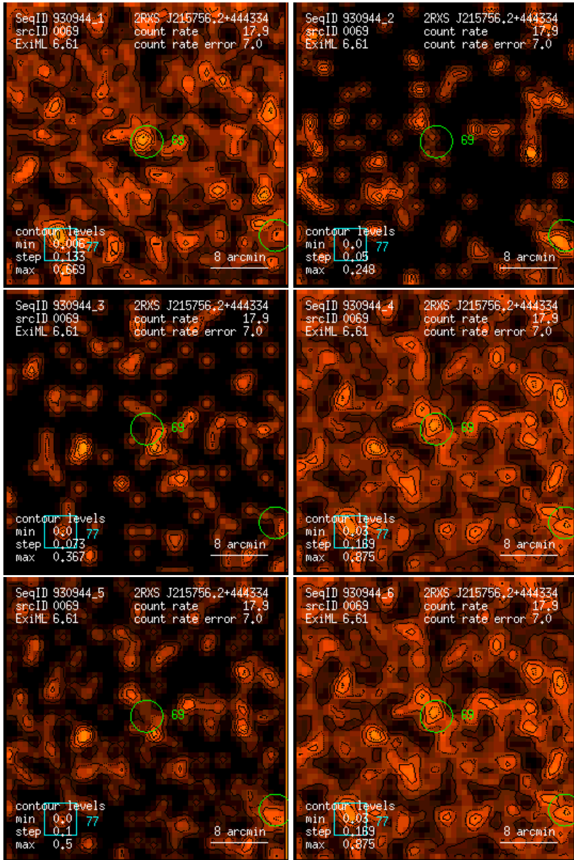
Figure 69: RASS 930944: detection 0069: band rate images, Gaussian filter: (1) PSPC channels 11 – 41, (2) 52 – 90, (3) 91 – 201, (4) 11 – 235, (5) 52 – 201, (6) 11 – 201. Broad band rates in counts/ks. Band rate contour levels in counts/ks/arcmin 2 .
