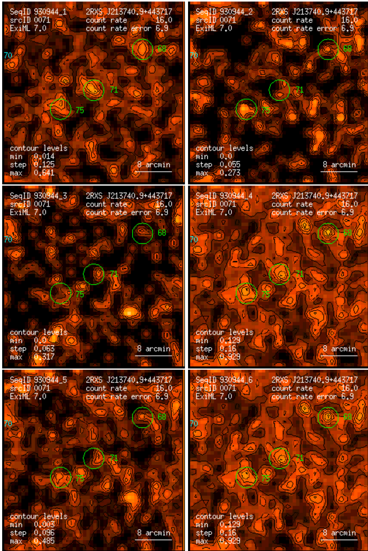
Figure 71: RASS 930944: detection 0071: band rate images, Gaussian filter: (1) PSPC channels 11 – 41, (2) 52 – 90, (3) 91 – 201, (4) 11 – 235, (5) 52 – 201, (6) 11 – 201. Broad band rates in counts/ks. Band rate contour levels in counts/ks/arcmin 2 .
