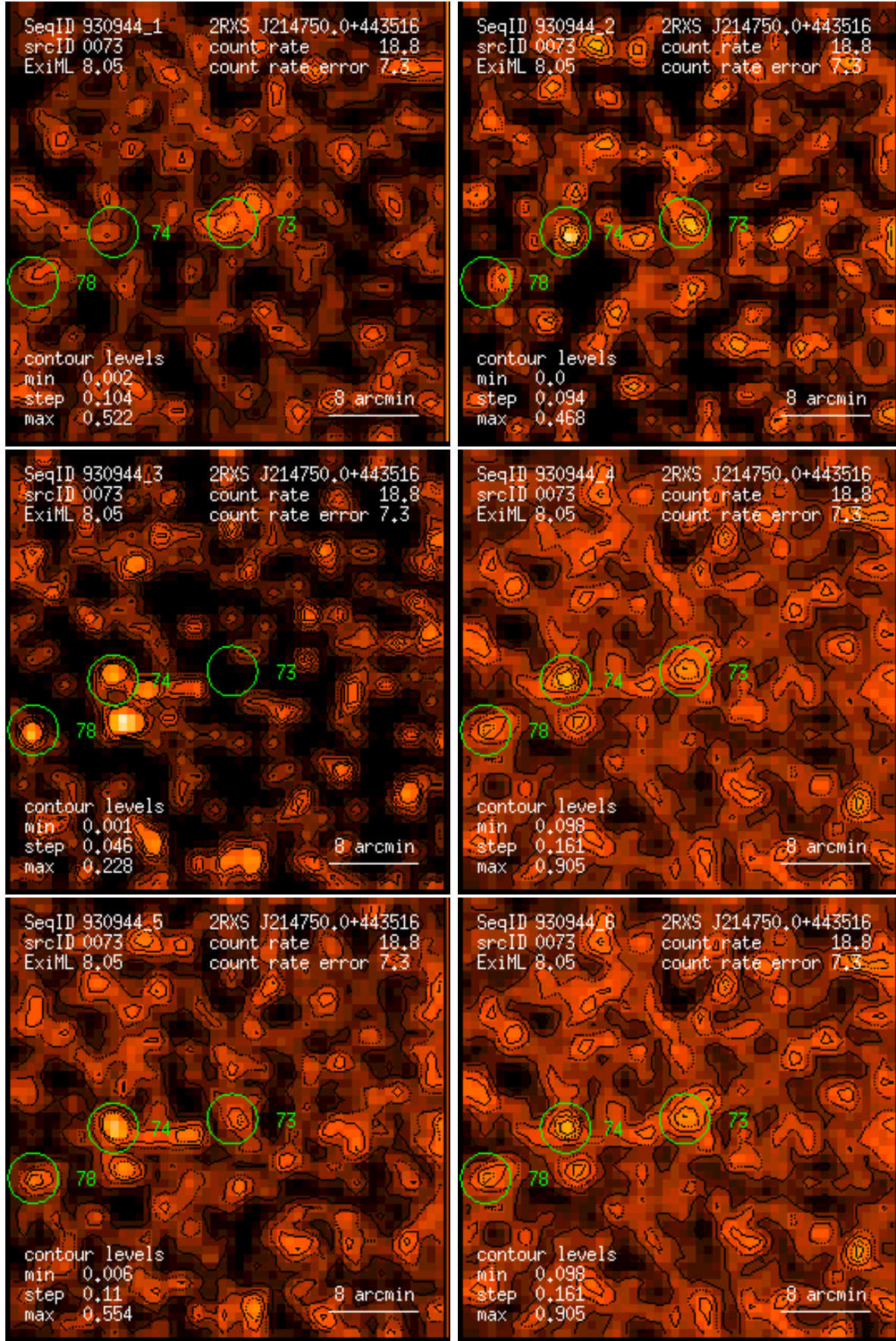
Figure 73: RASS 930944: detection 0073: band rate images, Gaussian filter: (1) PSPC channels 11 – 41, (2) 52 – 90, (3) 91 – 201, (4) 11 – 235, (5) 52 – 201, (6) 11 – 201. Broad band rates in counts/ks. Band rate contour levels in counts/ks/arcmin 2 .
