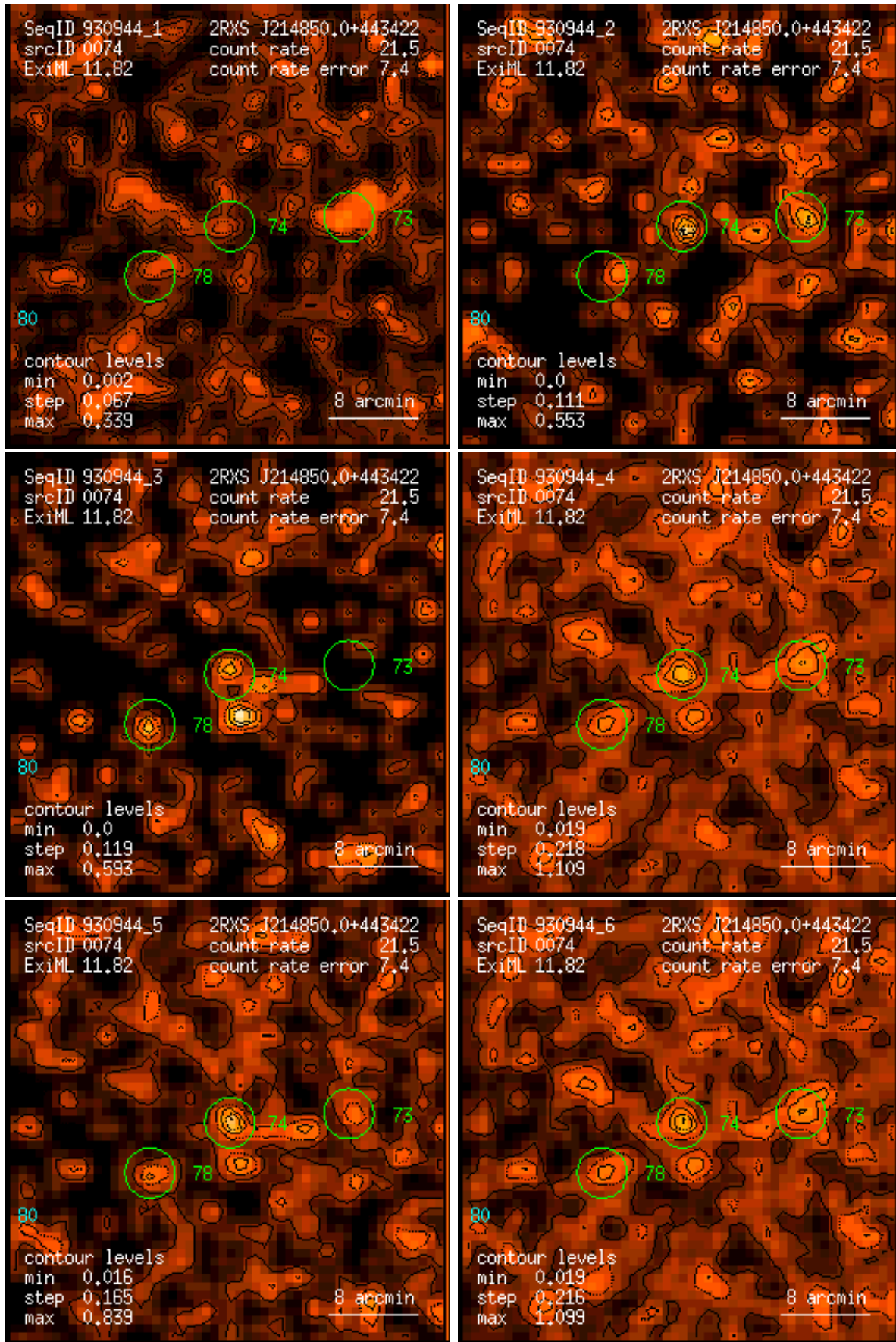
Figure 74: RASS 930944: detection 0074: band rate images, Gaussian filter: (1) PSPC channels 11 – 41, (2) 52 – 90, (3) 91 – 201, (4) 11 – 235, (5) 52 – 201, (6) 11 – 201. Broad band rates in counts/ks. Band rate contour levels in counts/ks/arcmin 2 .
