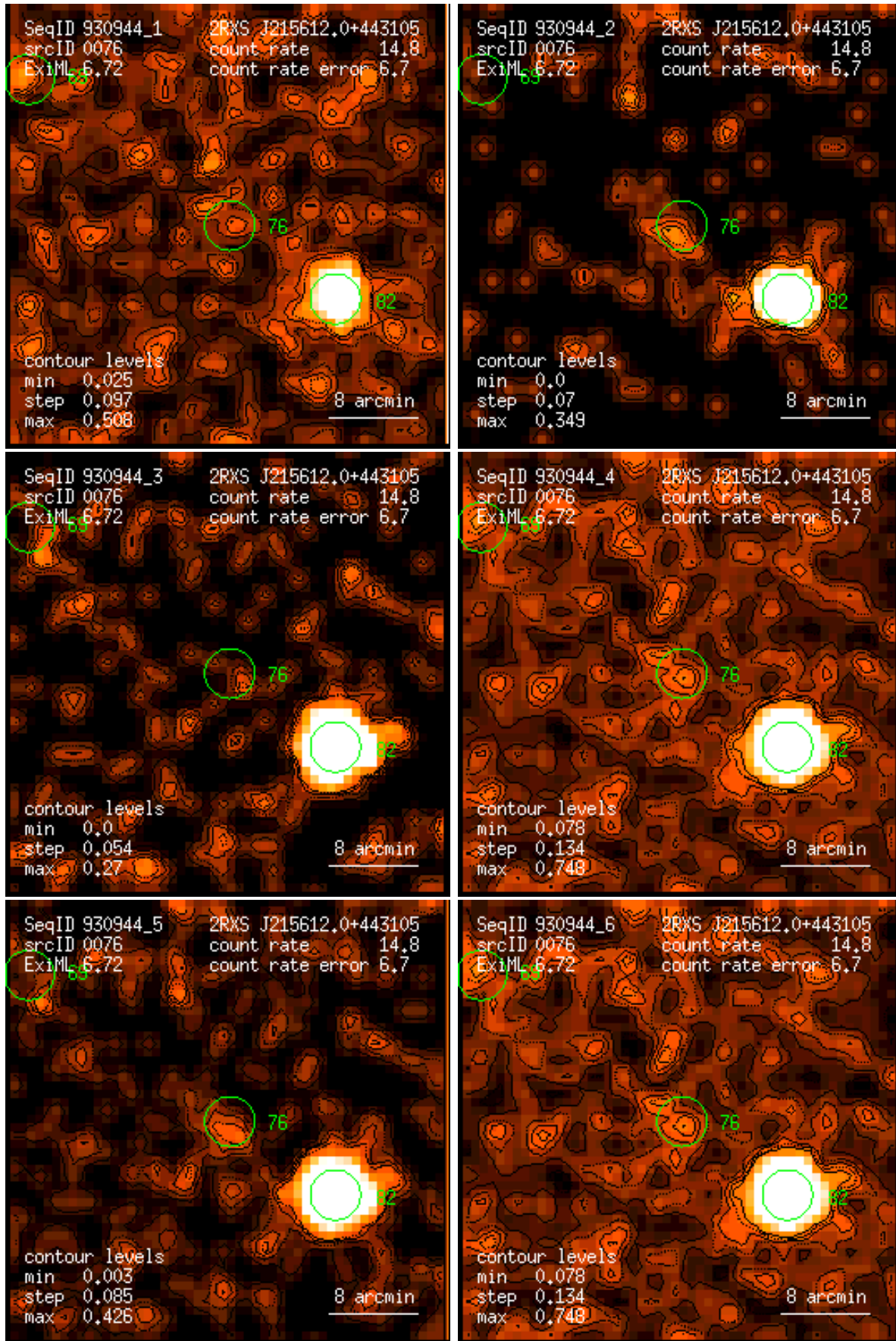
Figure 76: RASS 930944: detection 0076: band rate images, Gaussian filter: (1) PSPC channels 11 – 41, (2) 52 – 90, (3) 91 – 201, (4) 11 – 235, (5) 52 – 201, (6) 11 – 201. Broad band rates in counts/ks. Band rate contour levels in counts/ks/arcmin 2 .
