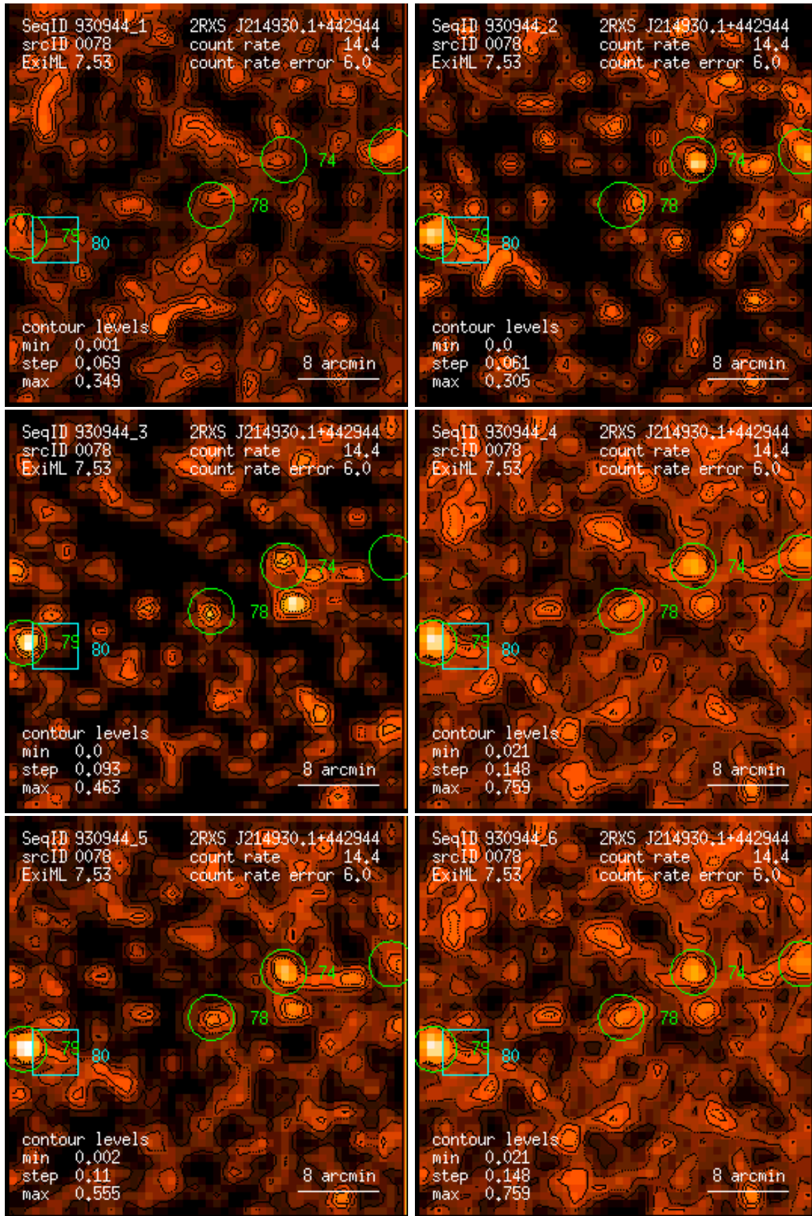
Figure 78: RASS 930944: detection 0078: band rate images, Gaussian filter: (1) PSPC channels 11 – 41, (2) 52 – 90, (3) 91 – 201, (4) 11 – 235, (5) 52 – 201, (6) 11 – 201. Broad band rates in counts/ks. Band rate contour levels in counts/ks/arcmin 2 .
