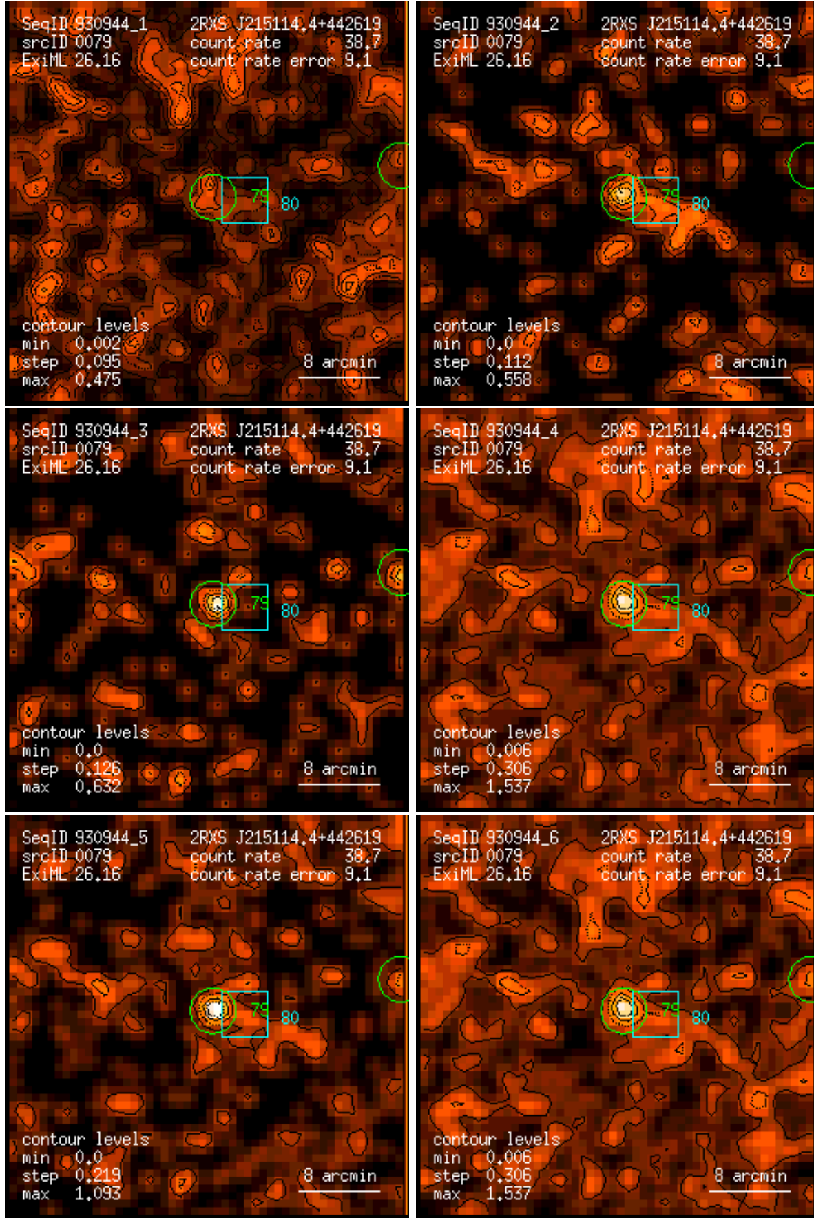
Figure 79: RASS 930944: detection 0079: band rate images, Gaussian filter: (1) PSPC channels 11 – 41, (2) 52 – 90, (3) 91 – 201, (4) 11 – 235, (5) 52 – 201, (6) 11 – 201. Broad band rates in counts/ks. Band rate contour levels in counts/ks/arcmin 2 .
