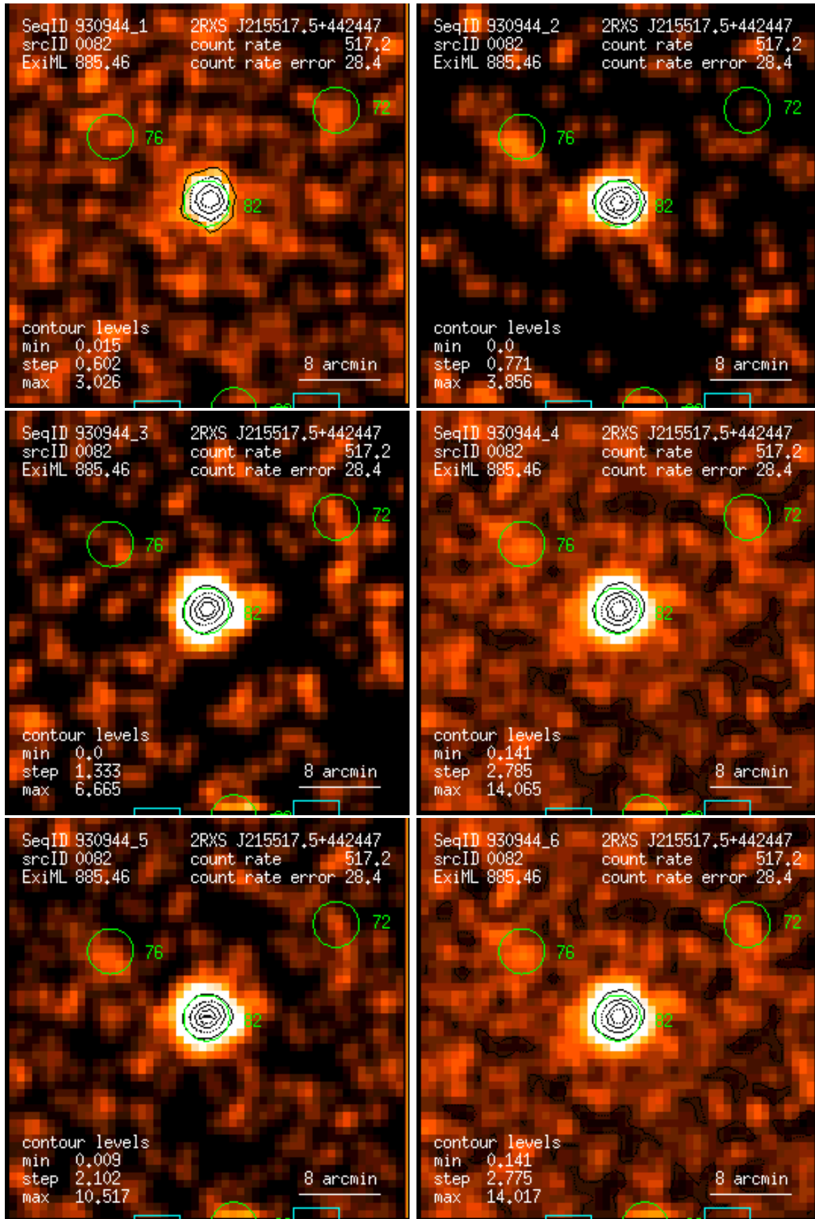
Figure 82: RASS 930944: detection 0082: band rate images, Gaussian filter: (1) PSPC channels 11 – 41, (2) 52 – 90, (3) 91 – 201, (4) 11 – 235, (5) 52 – 201, (6) 11 – 201. Broad band rates in counts/ks. Band rate contour levels in counts/ks/arcmin 2 .
