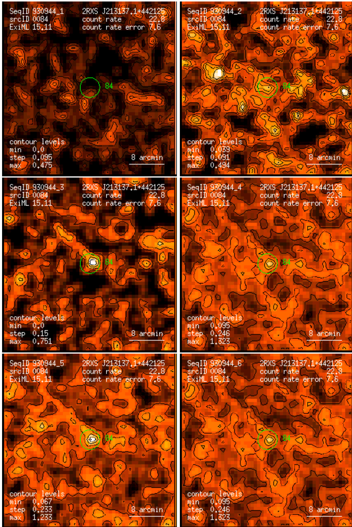
Figure 84: RASS 930944: detection 0084: band rate images, Gaussian filter: (1) PSPC channels 11 – 41, (2) 52 – 90, (3) 91 – 201, (4) 11 – 235, (5) 52 – 201, (6) 11 – 201. Broad band rates in counts/ks. Band rate contour levels in counts/ks/arcmin 2 .
