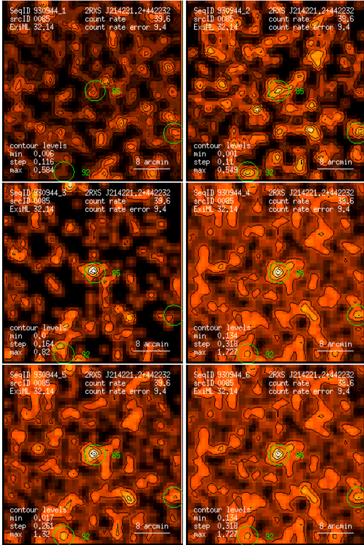
Figure 85: RASS 930944: detection 0085: band rate images, Gaussian filter: (1) PSPC channels 11 – 41, (2) 52 – 90, (3) 91 – 201, (4) 11 – 235, (5) 52 – 201, (6) 11 – 201. Broad band rates in counts/ks. Band rate contour levels in counts/ks/arcmin 2 .
