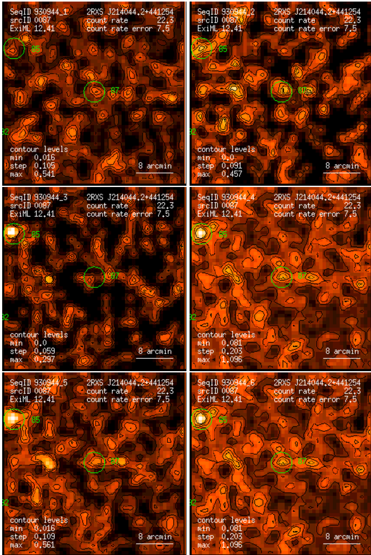
Figure 87: RASS 930944: detection 0087: band rate images, Gaussian filter: (1) PSPC channels 11 – 41, (2) 52 – 90, (3) 91 – 201, (4) 11 – 235, (5) 52 – 201, (6) 11 – 201. Broad band rates in counts/ks. Band rate contour levels in counts/ks/arcmin 2 .
