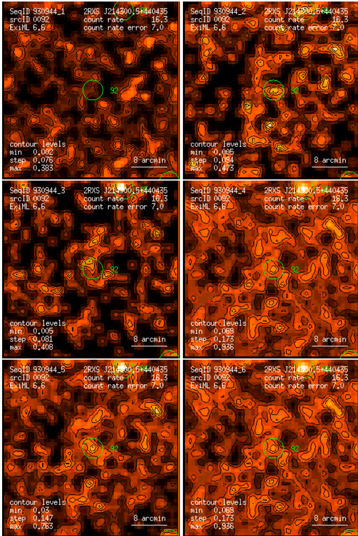
Figure 92: RASS 930944: detection 0092: band rate images, Gaussian filter: (1) PSPC channels 11 – 41, (2) 52 – 90, (3) 91 – 201, (4) 11 – 235, (5) 52 – 201, (6) 11 – 201. Broad band rates in counts/ks. Band rate contour levels in counts/ks/arcmin 2 .
