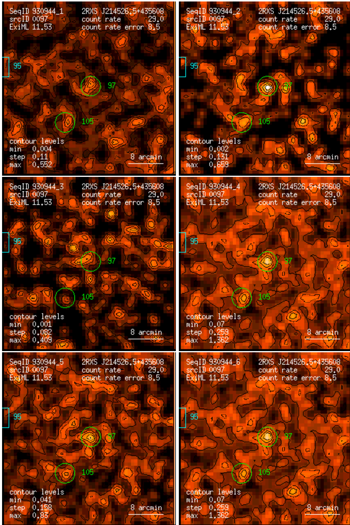
Figure 97: RASS 930944: detection 0097: band rate images, Gaussian filter: (1) PSPC channels 11 – 41, (2) 52 – 90, (3) 91 – 201, (4) 11 – 235, (5) 52 – 201, (6) 11 – 201. Broad band rates in counts/ks. Band rate contour levels in counts/ks/arcmin 2 .
