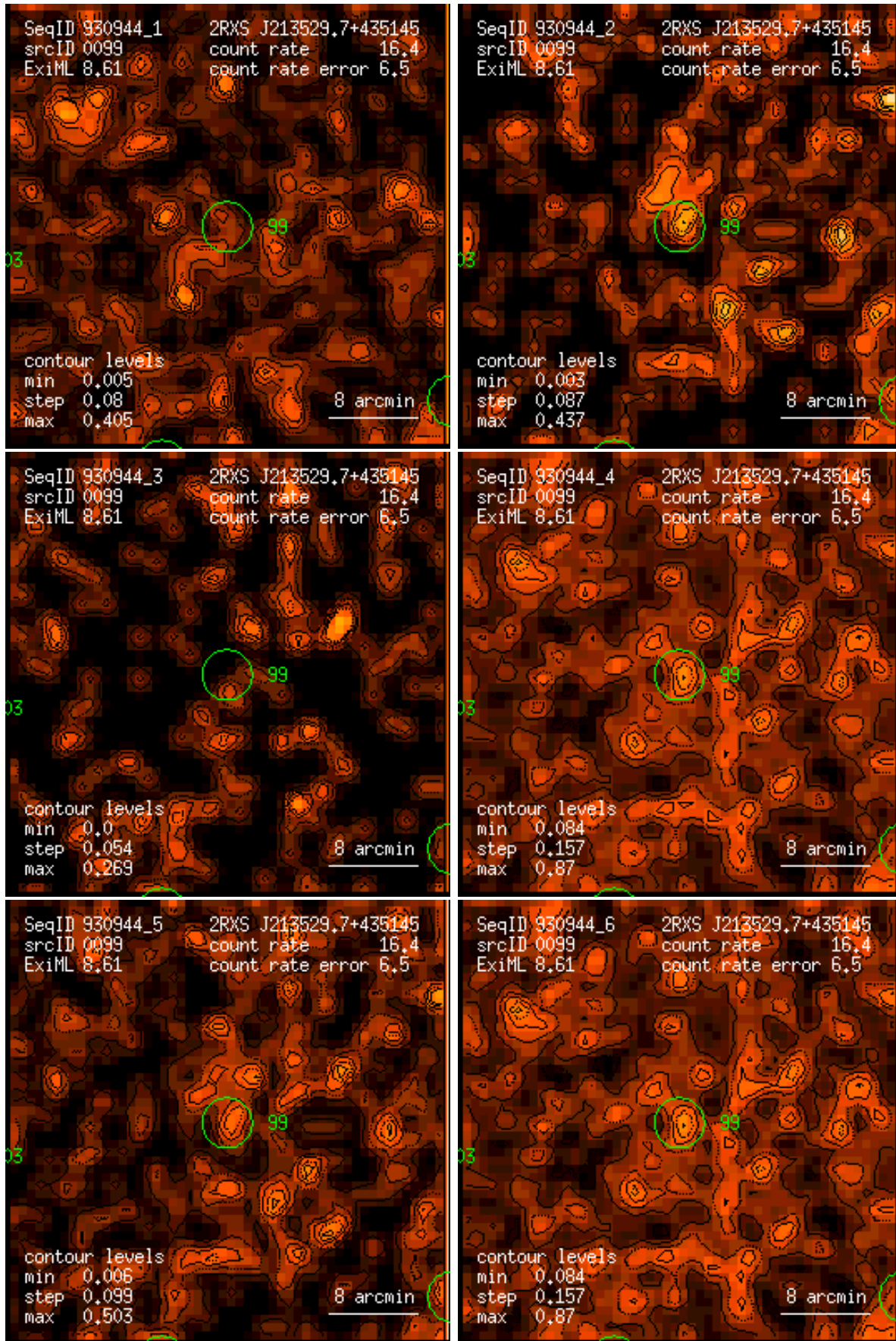
Figure 99: RASS 930944: detection 0099: band rate images, Gaussian filter: (1) PSPC channels 11 – 41, (2) 52 – 90, (3) 91 – 201, (4) 11 – 235, (5) 52 – 201, (6) 11 – 201. Broad band rates in counts/ks. Band rate contour levels in counts/ks/arcmin 2 .
