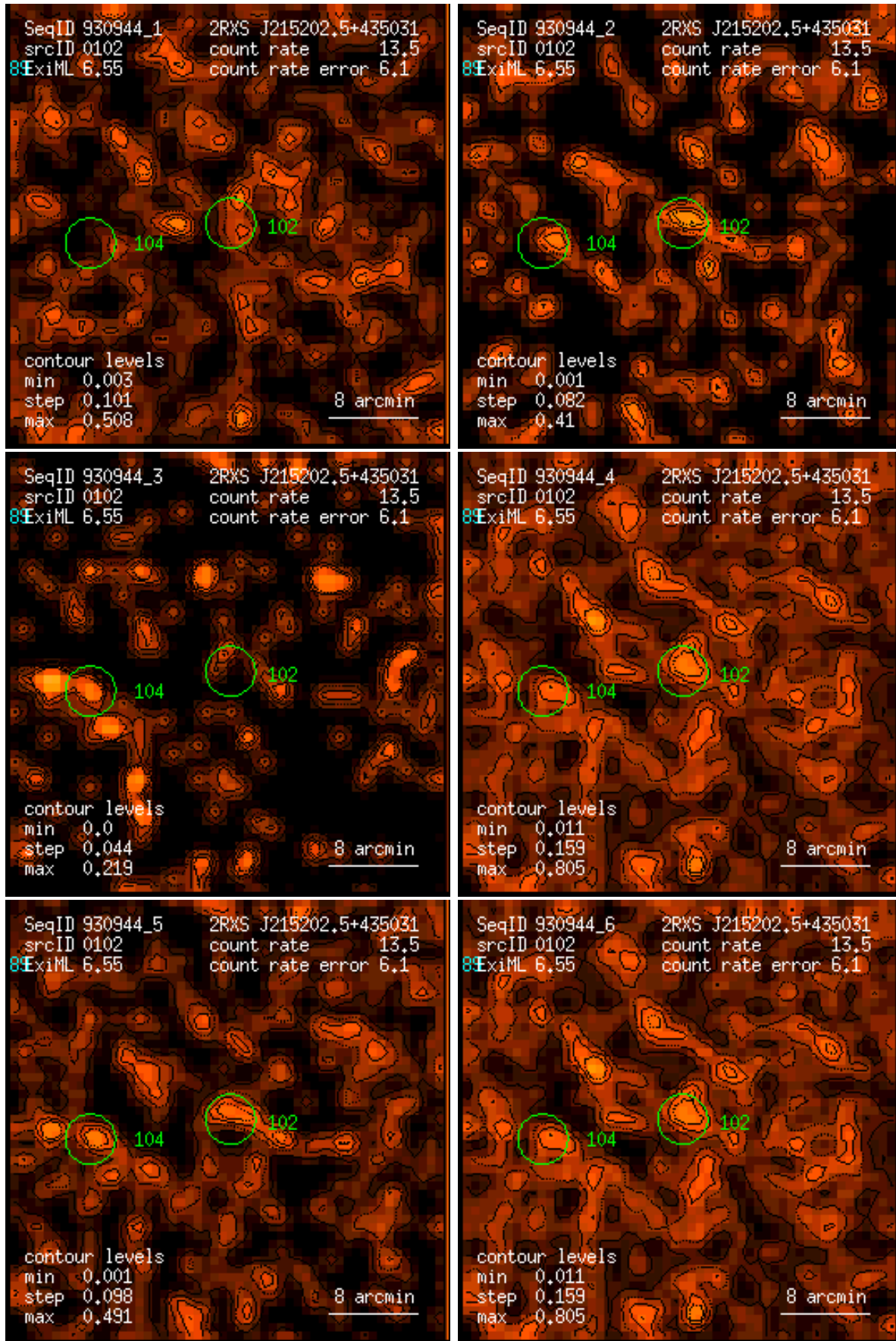
Figure 102: RASS 930944: detection 0102: band rate images, Gaussian filter: (1) PSPC channels 11 – 41, (2) 52 – 90, (3) 91 – 201, (4) 11 – 235, (5) 52 – 201, (6) 11 – 201. Broad band rates in counts/ks. Band rate contour levels in counts/ks/arcmin 2 .
