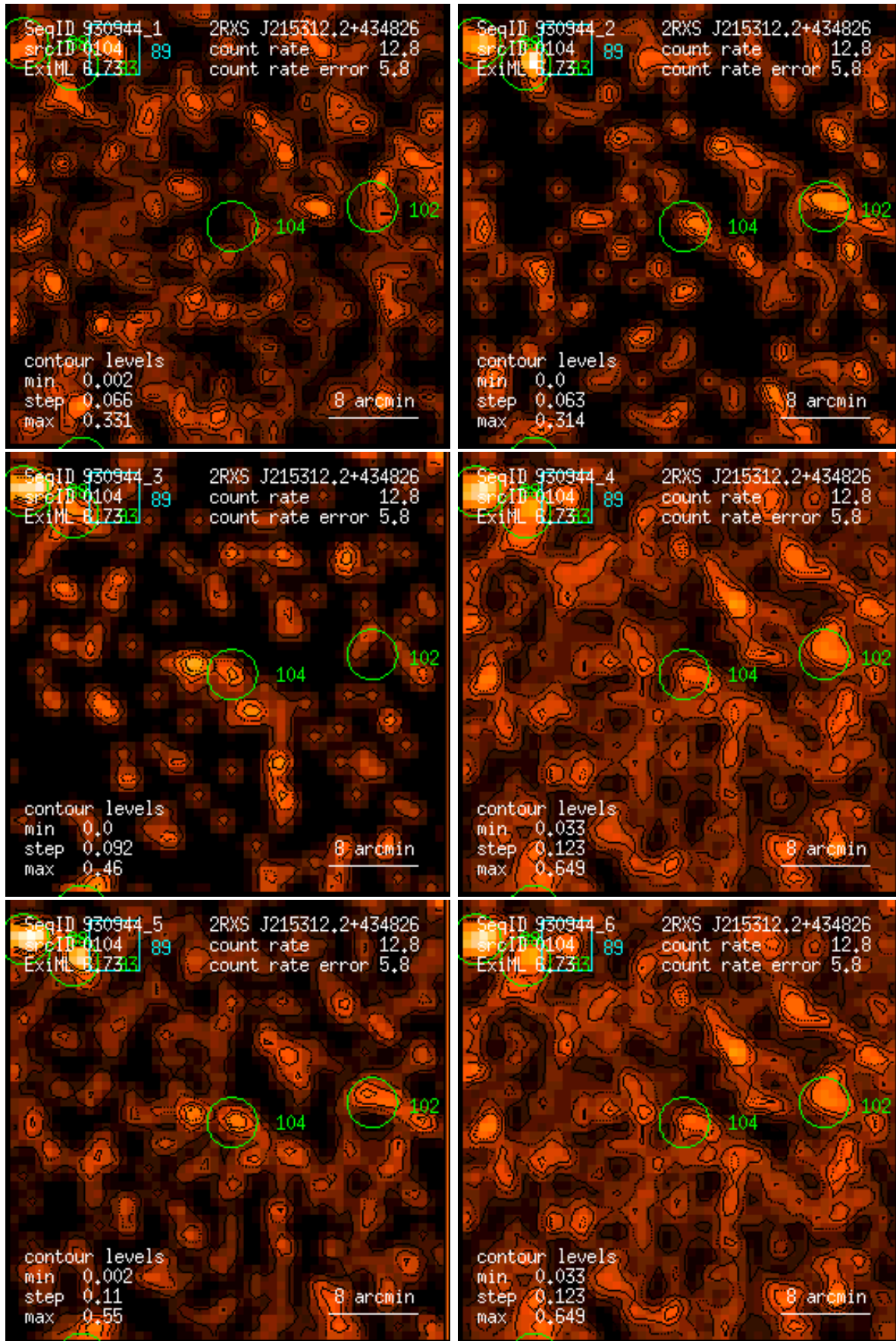
Figure 104: RASS 930944: detection 0104: band rate images, Gaussian filter: (1) PSPC channels 11 – 41, (2) 52 – 90, (3) 91 – 201, (4) 11 – 235, (5) 52 – 201, (6) 11 – 201. Broad band rates in counts/ks. Band rate contour levels in counts/ks/arcmin 2 .
