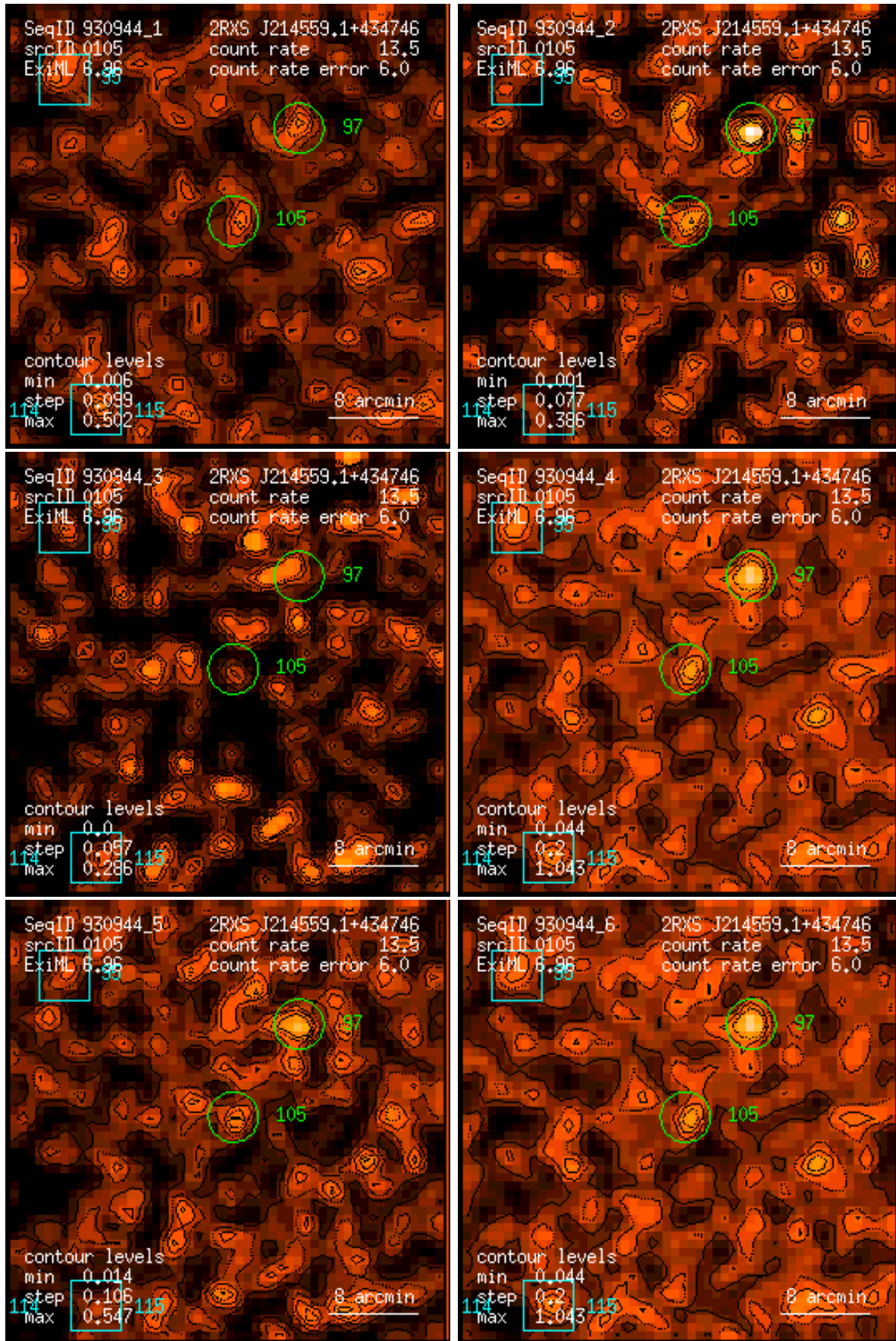
Figure 105: RASS 930944: detection 0105: band rate images, Gaussian filter: (1) PSPC channels 11 – 41, (2) 52 – 90, (3) 91 – 201, (4) 11 – 235, (5) 52 – 201, (6) 11 – 201. Broad band rates in counts/ks. Band rate contour levels in counts/ks/arcmin 2 .
