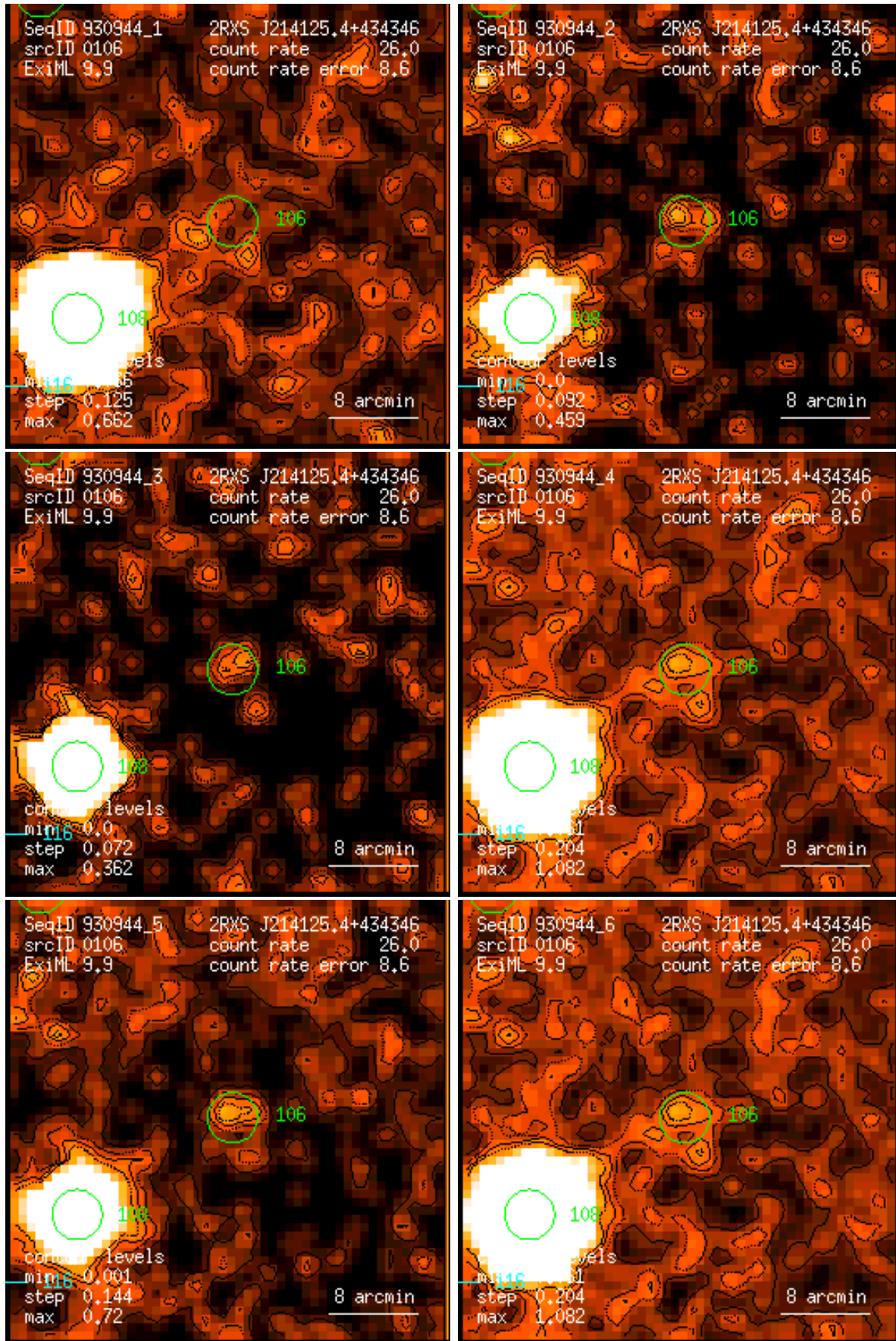
Figure 106: RASS 930944: detection 0106: band rate images, Gaussian filter: (1) PSPC channels 11 – 41, (2) 52 – 90, (3) 91 – 201, (4) 11 – 235, (5) 52 – 201, (6) 11 – 201. Broad band rates in counts/ks. Band rate contour levels in counts/ks/arcmin 2 .
