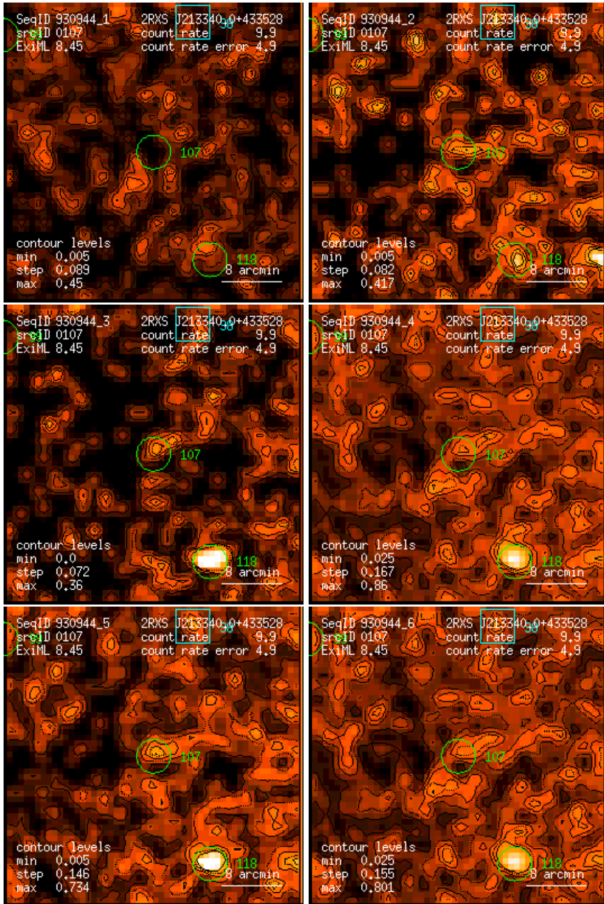
Figure 107: RASS 930944: detection 0107: band rate images, Gaussian filter: (1) PSPC channels 11 – 41, (2) 52 – 90, (3) 91 – 201, (4) 11 – 235, (5) 52 – 201, (6) 11 – 201. Broad band rates in counts/ks. Band rate contour levels in counts/ks/arcmin 2 .
