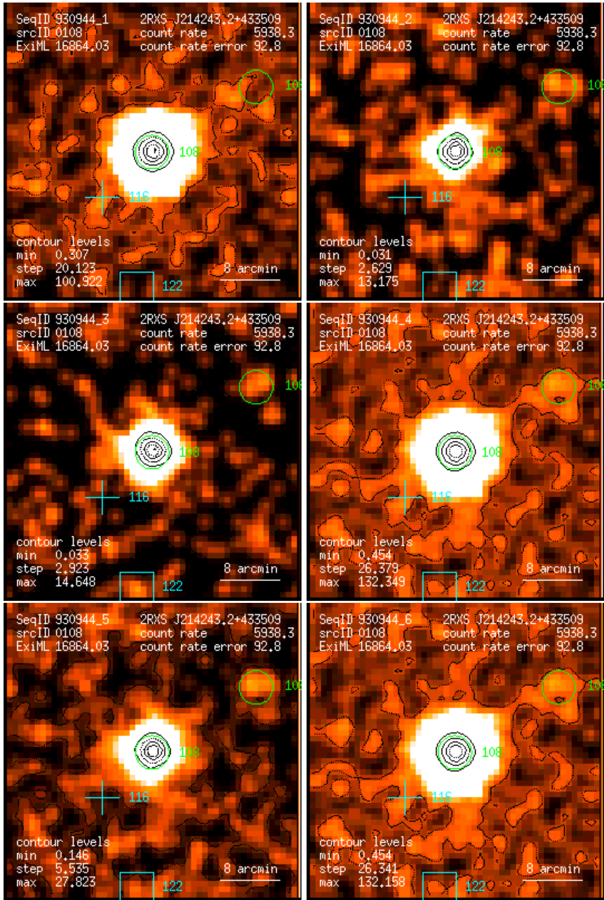
Figure 108: RASS 930944: detection 0108: band rate images, Gaussian filter: (1) PSPC channels 11 – 41, (2) 52 – 90, (3) 91 – 201, (4) 11 – 235, (5) 52 – 201, (6) 11 – 201. Broad band rates in counts/ks. Band rate contour levels in counts/ks/arcmin 2 .
