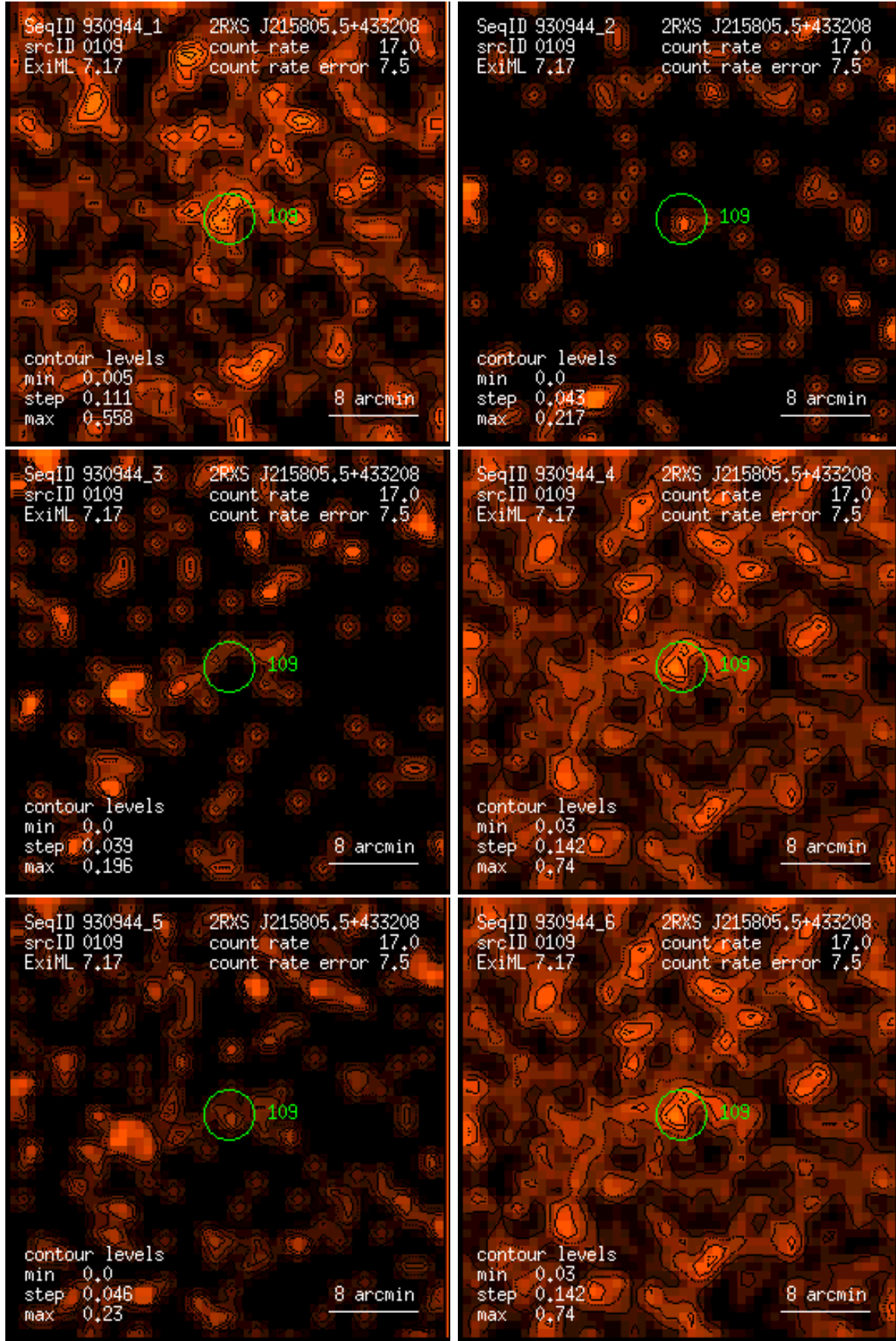
Figure 109: RASS 930944: detection 0109: band rate images, Gaussian filter: (1) PSPC channels 11 – 41, (2) 52 – 90, (3) 91 – 201, (4) 11 – 235, (5) 52 – 201, (6) 11 – 201. Broad band rates in counts/ks. Band rate contour levels in counts/ks/arcmin 2 .
