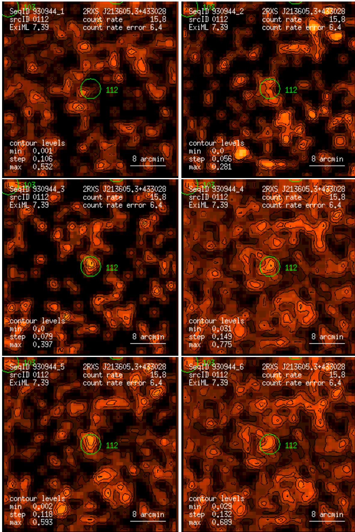
Figure 112: RASS 930944: detection 0112: band rate images, Gaussian filter: (1) PSPC channels 11 – 41, (2) 52 – 90, (3) 91 – 201, (4) 11 – 235, (5) 52 – 201, (6) 11 – 201. Broad band rates in counts/ks. Band rate contour levels in counts/ks/arcmin 2 .
