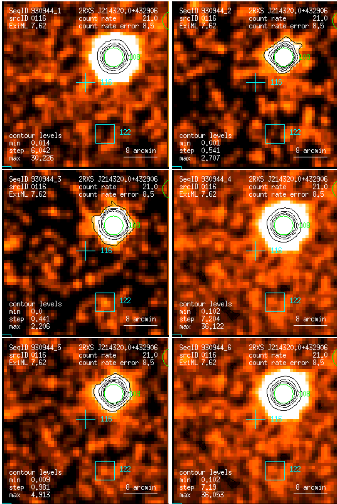
Figure 116: RASS 930944: detection 0116: band rate images, Gaussian filter: (1) PSPC channels 11 – 41, (2) 52 – 90, (3) 91 – 201, (4) 11 – 235, (5) 52 – 201, (6) 11 – 201. Broad band rates in counts/ks. Band rate contour levels in counts/ks/arcmin 2 .
