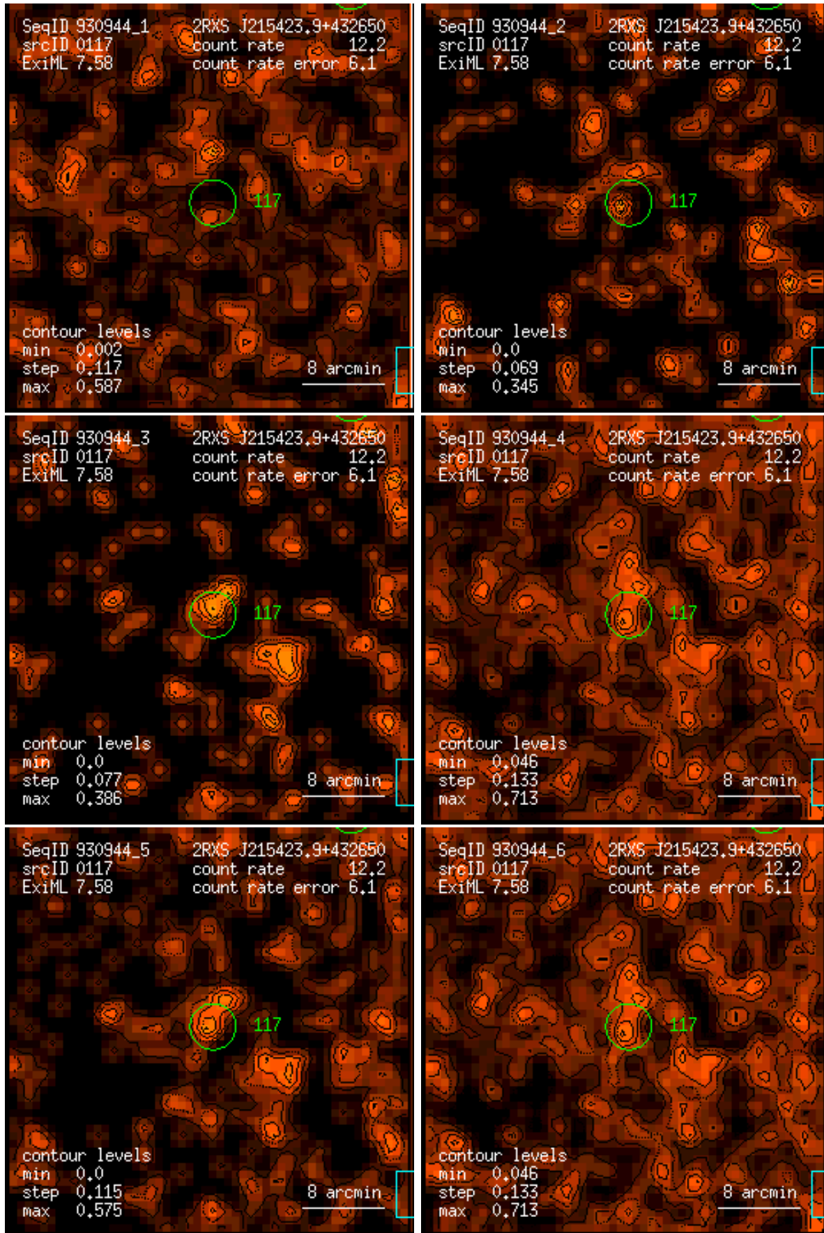
Figure 117: RASS 930944: detection 0117: band rate images, Gaussian filter: (1) PSPC channels 11 – 41, (2) 52 – 90, (3) 91 – 201, (4) 11 – 235, (5) 52 – 201, (6) 11 – 201. Broad band rates in counts/ks. Band rate contour levels in counts/ks/arcmin 2 .
