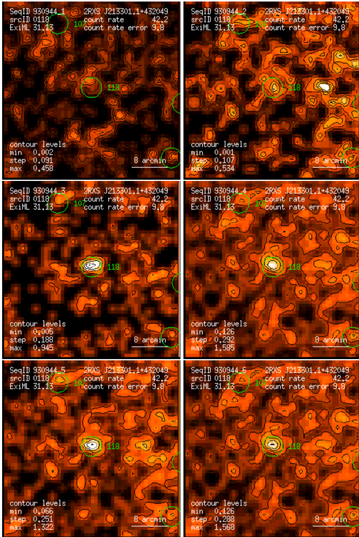
Figure 118: RASS 930944: detection 0118: band rate images, Gaussian filter: (1) PSPC channels 11 – 41, (2) 52 – 90, (3) 91 – 201, (4) 11 – 235, (5) 52 – 201, (6) 11 – 201. Broad band rates in counts/ks. Band rate contour levels in counts/ks/arcmin 2 .
