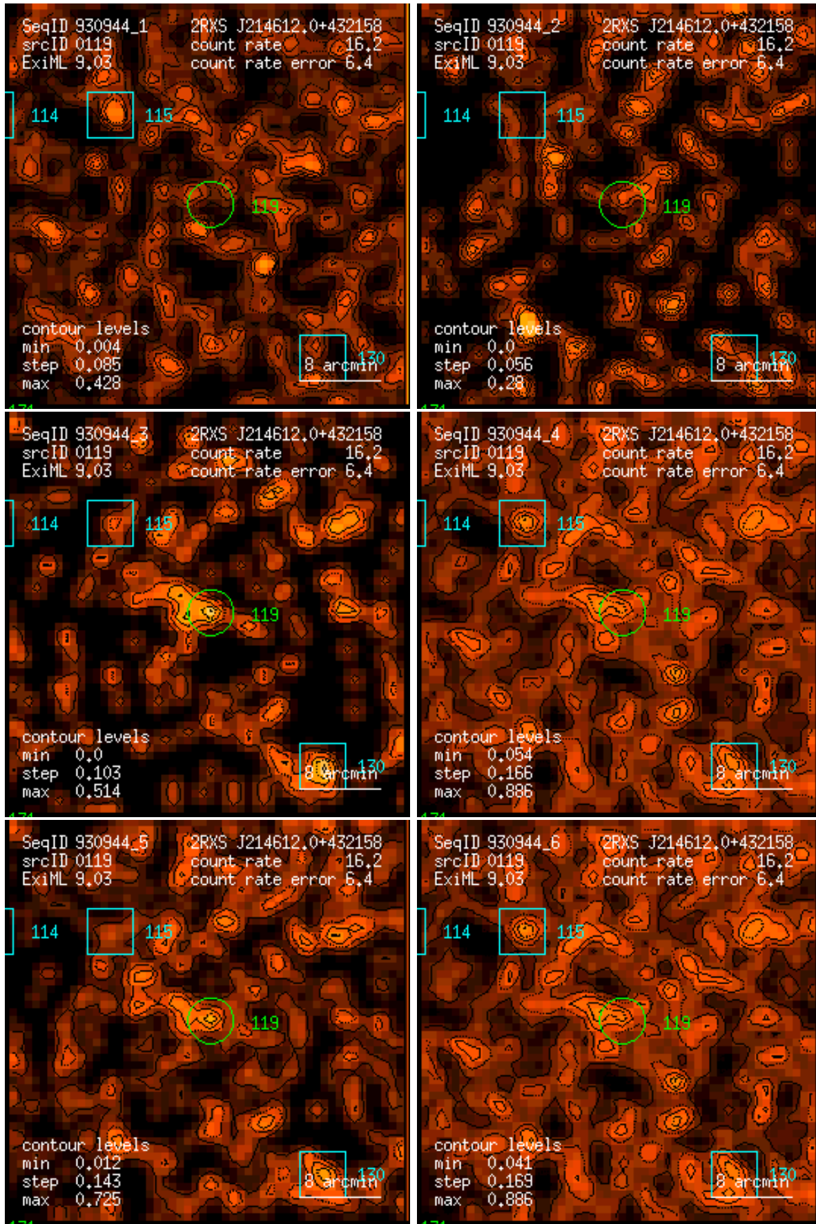
Figure 119: RASS 930944: detection 0119: band rate images, Gaussian filter: (1) PSPC channels 11 – 41, (2) 52 – 90, (3) 91 – 201, (4) 11 – 235, (5) 52 – 201, (6) 11 – 201. Broad band rates in counts/ks. Band rate contour levels in counts/ks/arcmin 2 .
