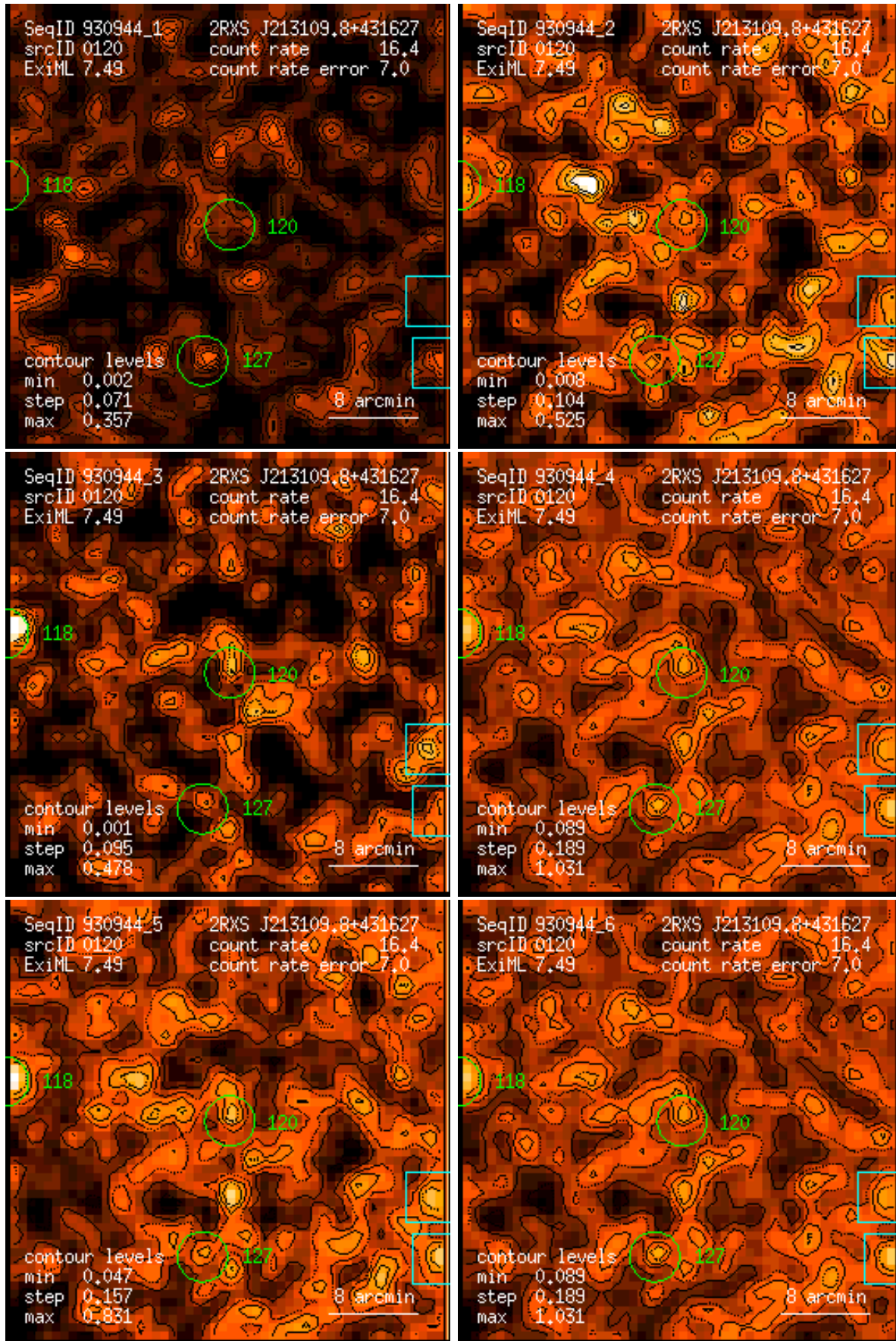
Figure 120: RASS 930944: detection 0120: band rate images, Gaussian filter: (1) PSPC channels 11 – 41, (2) 52 – 90, (3) 91 – 201, (4) 11 – 235, (5) 52 – 201, (6) 11 – 201. Broad band rates in counts/ks. Band rate contour levels in counts/ks/arcmin 2 .
