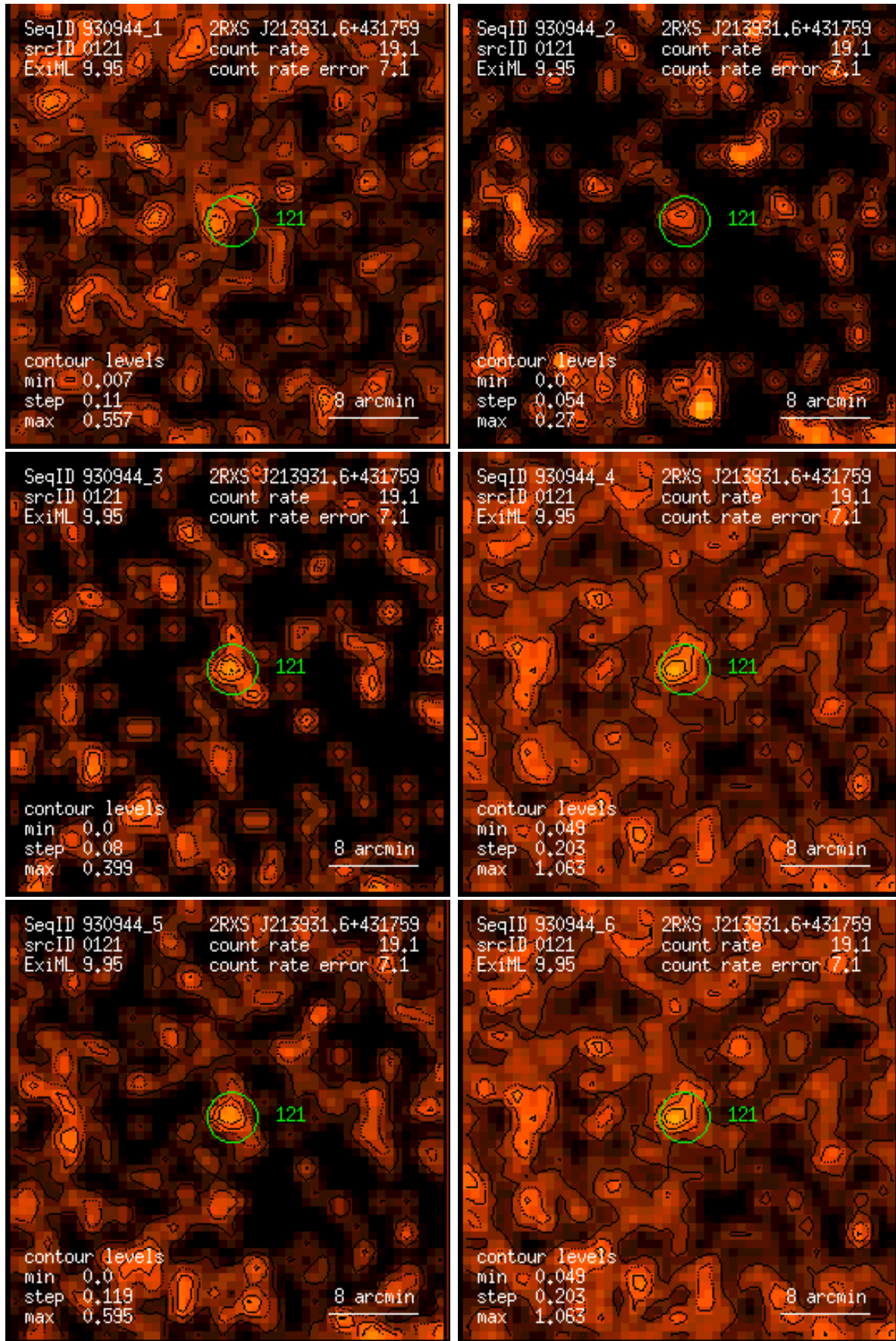
Figure 121: RASS 930944: detection 0121: band rate images, Gaussian filter: (1) PSPC channels 11 – 41, (2) 52 – 90, (3) 91 – 201, (4) 11 – 235, (5) 52 – 201, (6) 11 – 201. Broad band rates in counts/ks. Band rate contour levels in counts/ks/arcmin 2 .
