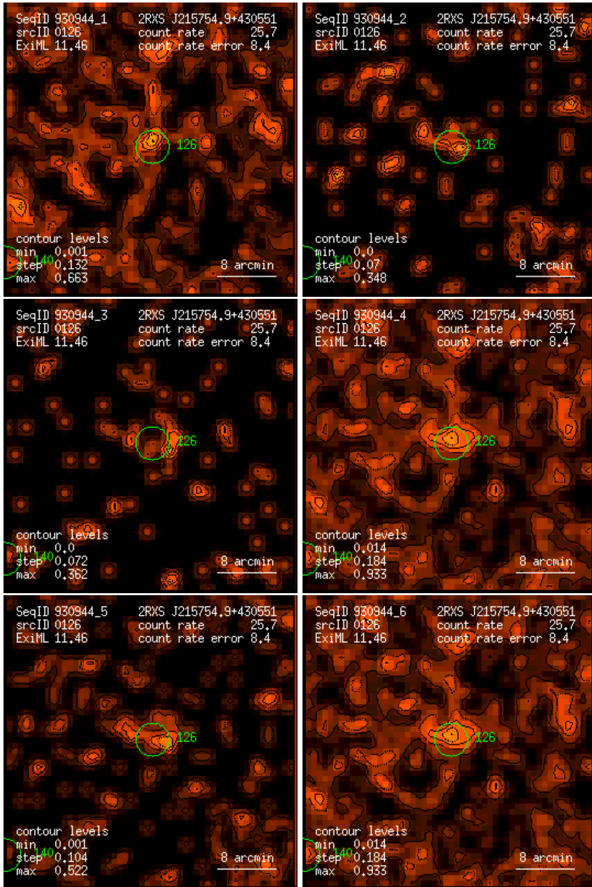
Figure 126: RASS 930944: detection 0126: band rate images, Gaussian filter: (1) PSPC channels 11 – 41, (2) 52 – 90, (3) 91 – 201, (4) 11 – 235, (5) 52 – 201, (6) 11 – 201. Broad band rates in counts/ks. Band rate contour levels in counts/ks/arcmin 2 .
