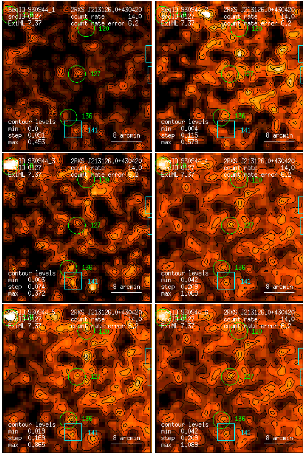
Figure 127: RASS 930944: detection 0127: band rate images, Gaussian filter: (1) PSPC channels 11 – 41, (2) 52 – 90, (3) 91 – 201, (4) 11 – 235, (5) 52 – 201, (6) 11 – 201. Broad band rates in counts/ks. Band rate contour levels in counts/ks/arcmin 2 .
