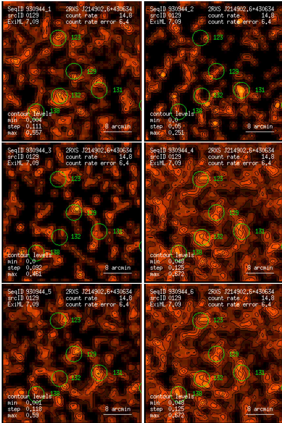
Figure 129: RASS 930944: detection 0129: band rate images, Gaussian filter: (1) PSPC channels 11 – 41, (2) 52 – 90, (3) 91 – 201, (4) 11 – 235, (5) 52 – 201, (6) 11 – 201. Broad band rates in counts/ks. Band rate contour levels in counts/ks/arcmin 2 .
