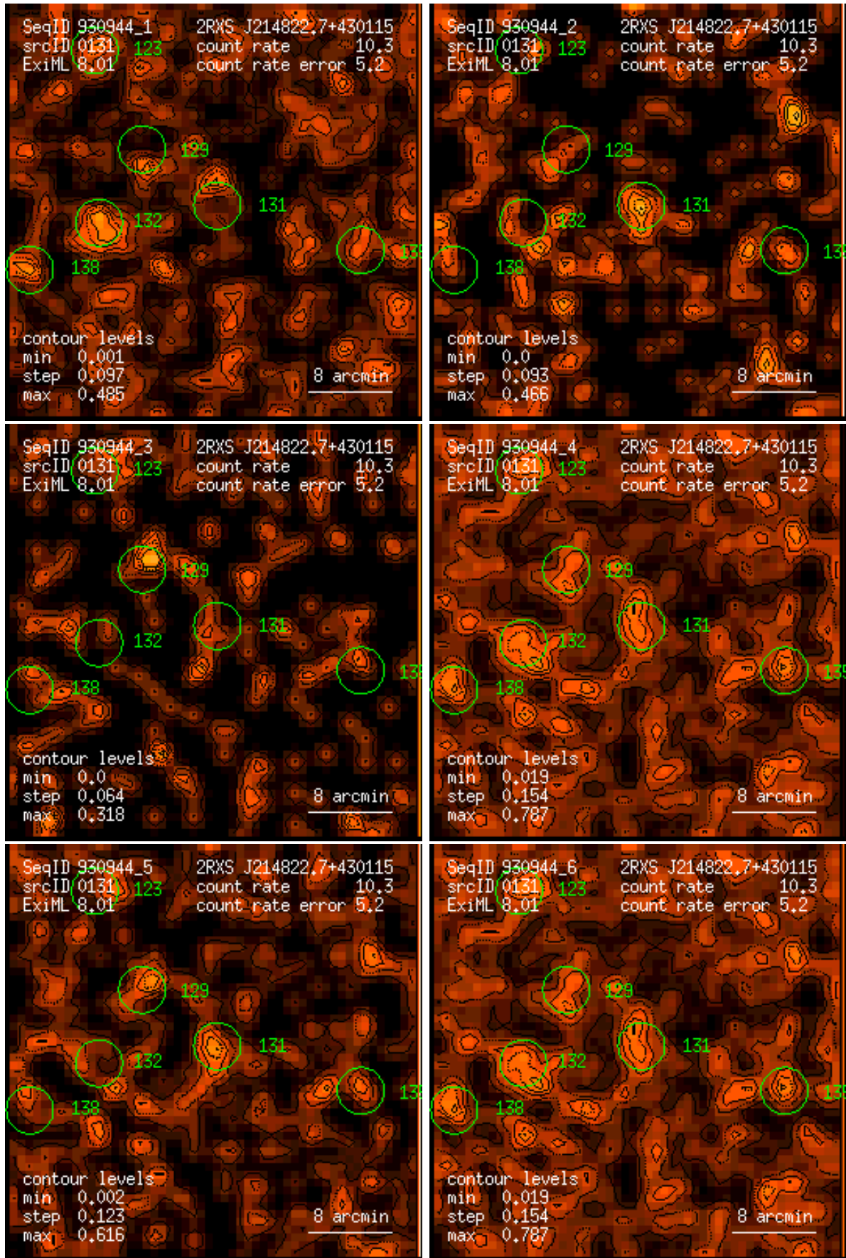
Figure 131: RASS 930944: detection 0131: band rate images, Gaussian filter: (1) PSPC channels 11 – 41, (2) 52 – 90, (3) 91 – 201, (4) 11 – 235, (5) 52 – 201, (6) 11 – 201. Broad band rates in counts/ks. Band rate contour levels in counts/ks/arcmin 2 .
