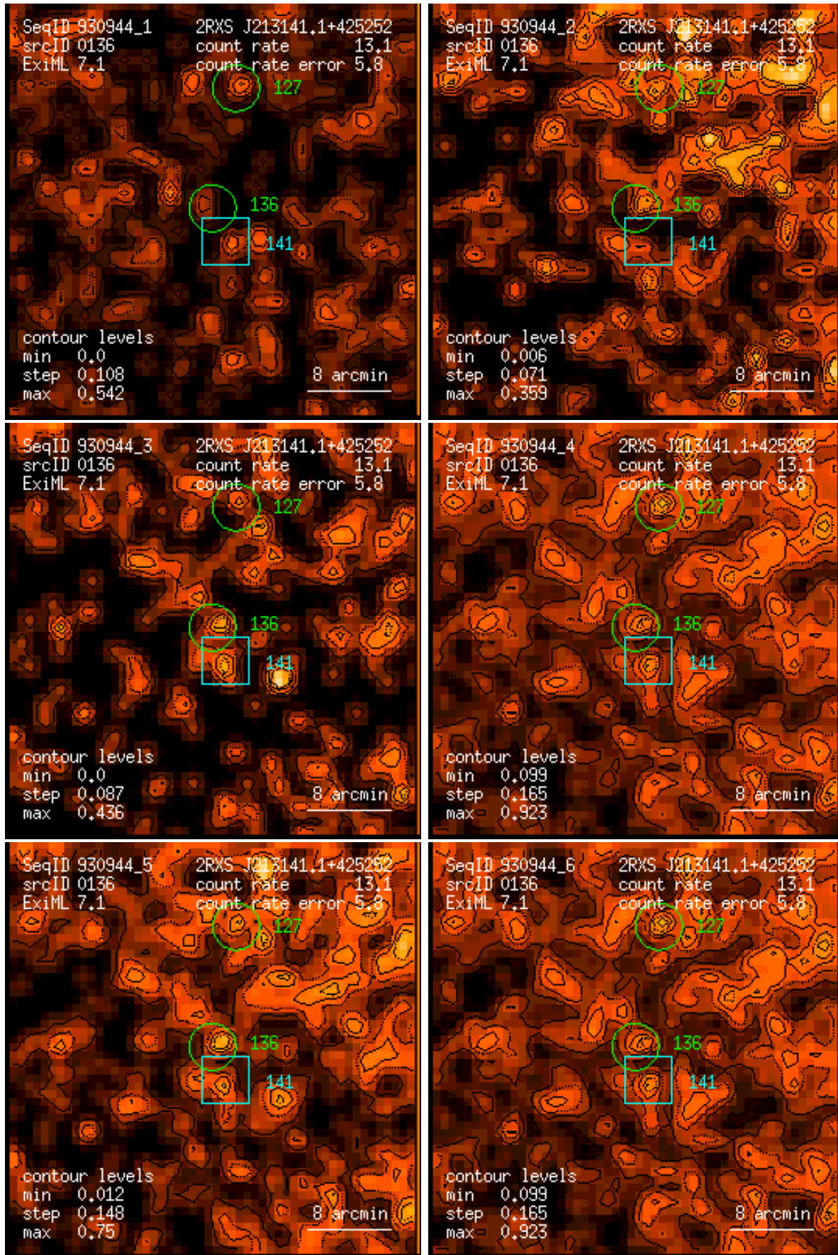
Figure 136: RASS 930944: detection 0136: band rate images, Gaussian filter: (1) PSPC channels 11 – 41, (2) 52 – 90, (3) 91 – 201, (4) 11 – 235, (5) 52 – 201, (6) 11 – 201. Broad band rates in counts/ks. Band rate contour levels in counts/ks/arcmin 2 .
