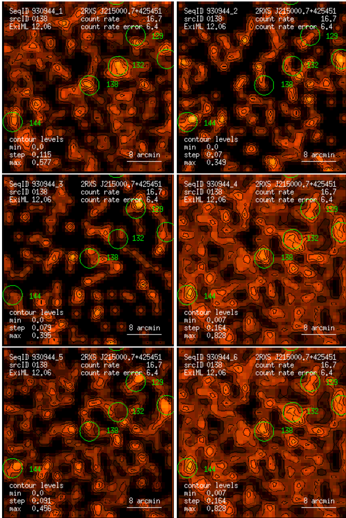
Figure 138: RASS 930944: detection 0138: band rate images, Gaussian filter: (1) PSPC channels 11 – 41, (2) 52 – 90, (3) 91 – 201, (4) 11 – 235, (5) 52 – 201, (6) 11 – 201. Broad band rates in counts/ks. Band rate contour levels in counts/ks/arcmin 2 .
