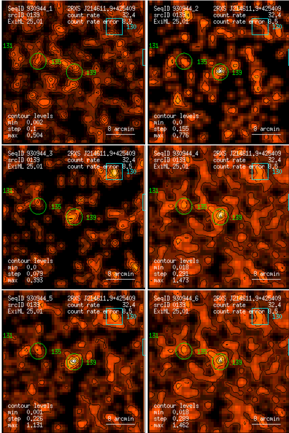
Figure 139: RASS 930944: detection 0139: band rate images, Gaussian filter: (1) PSPC channels 11 – 41, (2) 52 – 90, (3) 91 – 201, (4) 11 – 235, (5) 52 – 201, (6) 11 – 201. Broad band rates in counts/ks. Band rate contour levels in counts/ks/arcmin 2 .
