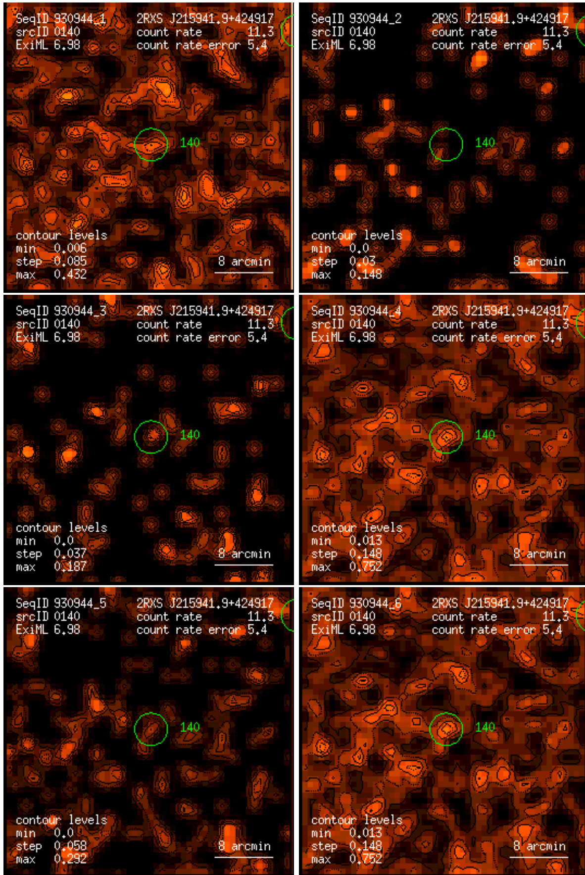
Figure 140: RASS 930944: detection 0140: band rate images, Gaussian filter: (1) PSPC channels 11 – 41, (2) 52 – 90, (3) 91 – 201, (4) 11 – 235, (5) 52 – 201, (6) 11 – 201. Broad band rates in counts/ks. Band rate contour levels in counts/ks/arcmin 2 .
