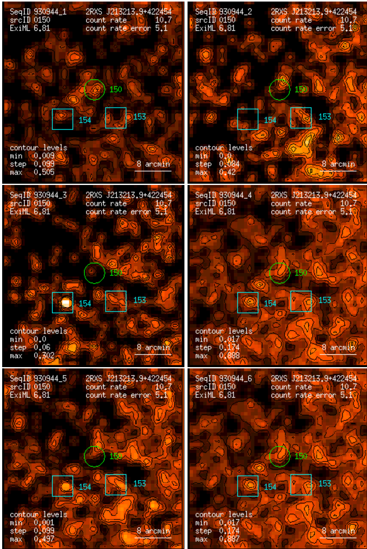
Figure 150: RASS 930944: detection 0150: band rate images, Gaussian filter: (1) PSPC channels 11 – 41, (2) 52 – 90, (3) 91 – 201, (4) 11 – 235, (5) 52 – 201, (6) 11 – 201. Broad band rates in counts/ks. Band rate contour levels in counts/ks/arcmin 2 .
