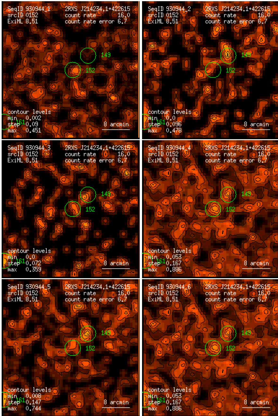
Figure 152: RASS 930944: detection 0152: band rate images, Gaussian filter: (1) PSPC channels 11 – 41, (2) 52 – 90, (3) 91 – 201, (4) 11 – 235, (5) 52 – 201, (6) 11 – 201. Broad band rates in counts/ks. Band rate contour levels in counts/ks/arcmin 2 .
