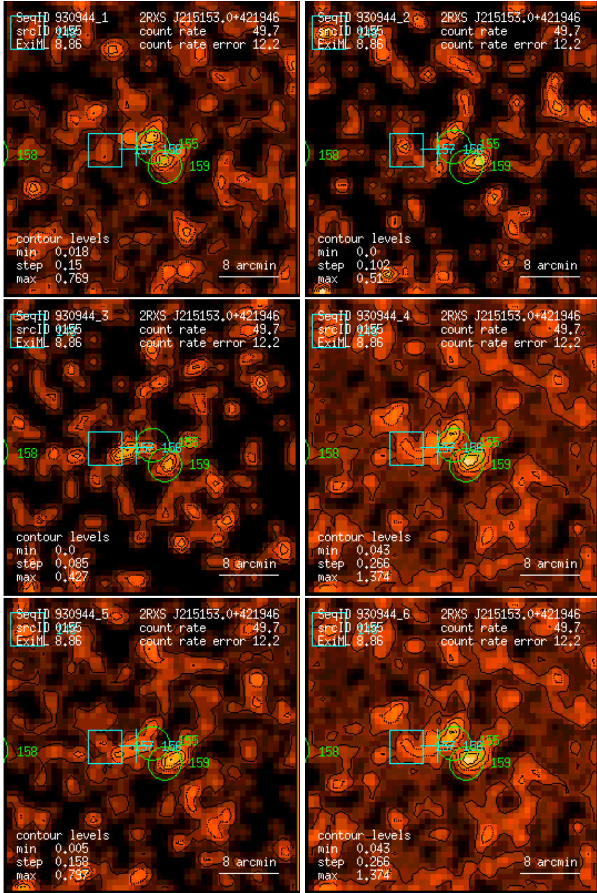
Figure 155: RASS 930944: detection 0155: band rate images, Gaussian filter: (1) PSPC channels 11 – 41, (2) 52 – 90, (3) 91 – 201, (4) 11 – 235, (5) 52 – 201, (6) 11 – 201. Broad band rates in counts/ks. Band rate contour levels in counts/ks/arcmin 2 .
