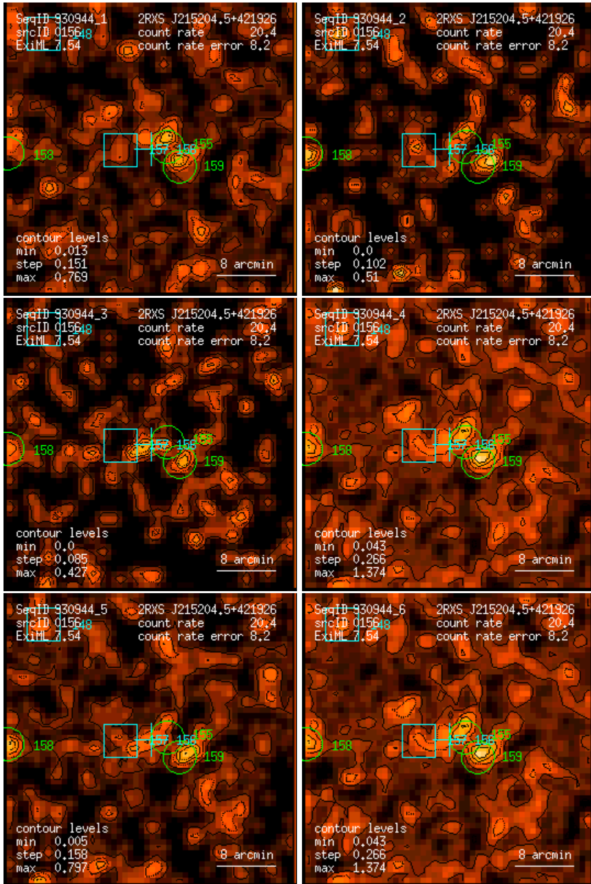
Figure 156: RASS 930944: detection 0156: band rate images, Gaussian filter: (1) PSPC channels 11 – 41, (2) 52 – 90, (3) 91 – 201, (4) 11 – 235, (5) 52 – 201, (6) 11 – 201. Broad band rates in counts/ks. Band rate contour levels in counts/ks/arcmin 2 .
