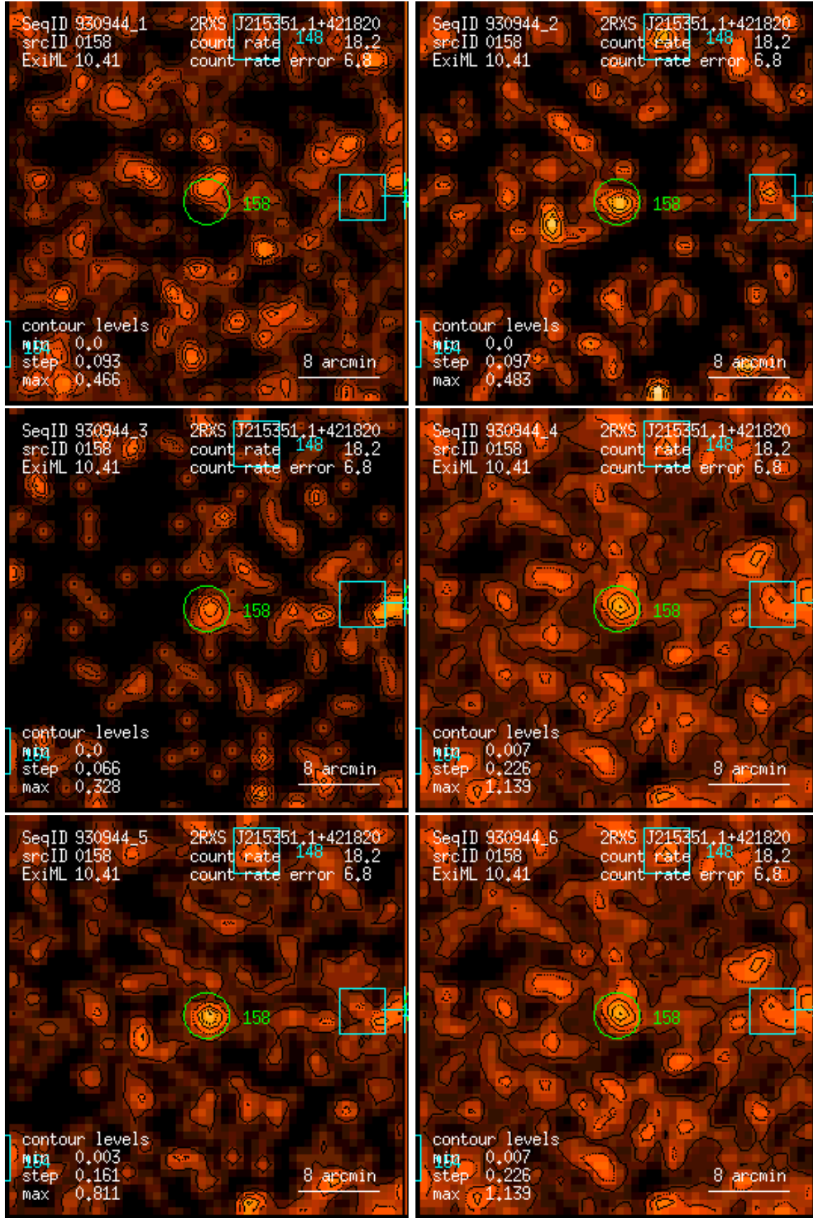
Figure 158: RASS 930944: detection 0158: band rate images, Gaussian filter: (1) PSPC channels 11 – 41, (2) 52 – 90, (3) 91 – 201, (4) 11 – 235, (5) 52 – 201, (6) 11 – 201. Broad band rates in counts/ks. Band rate contour levels in counts/ks/arcmin 2 .
