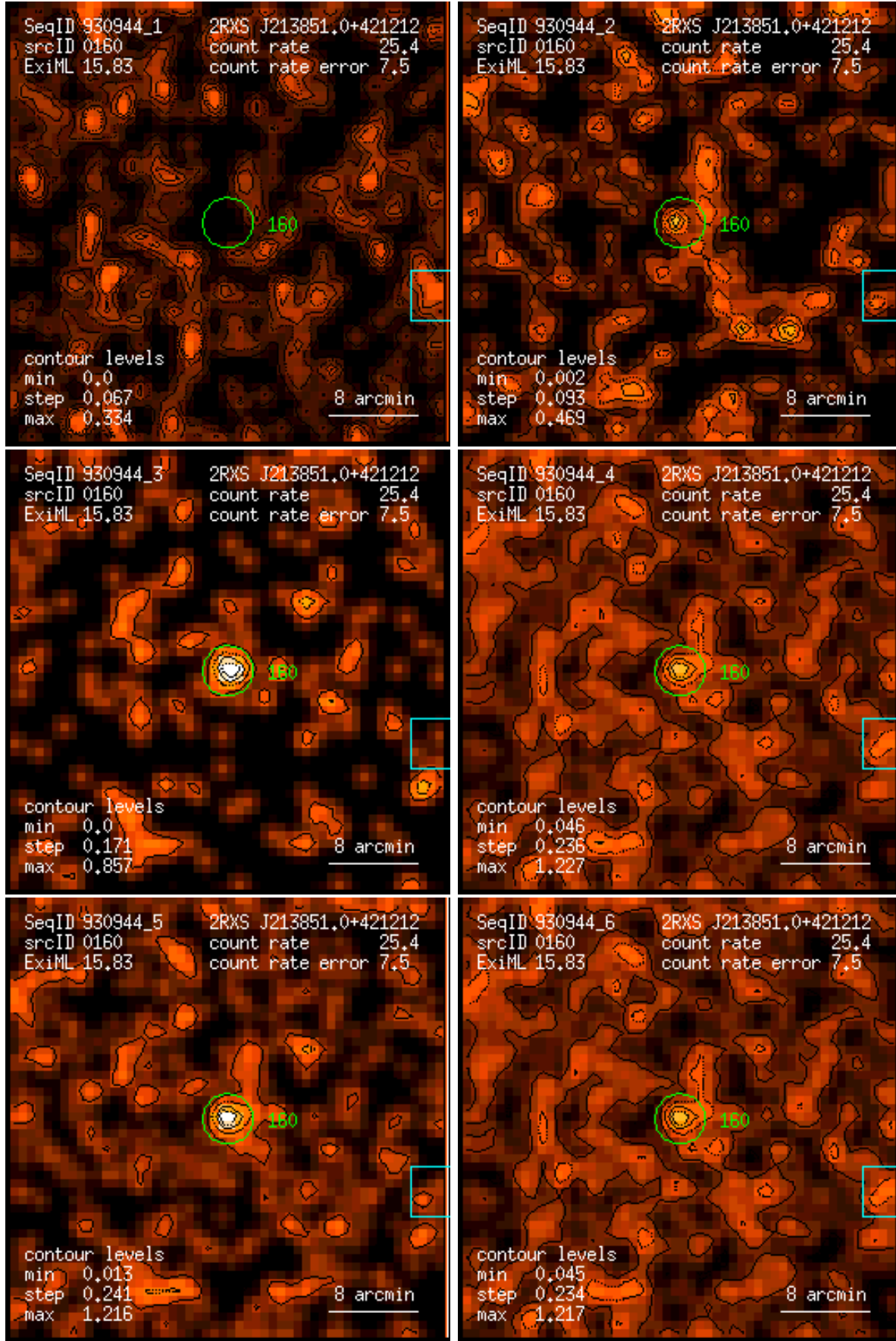
Figure 160: RASS 930944: detection 0160: band rate images, Gaussian filter: (1) PSPC channels 11 – 41, (2) 52 – 90, (3) 91 – 201, (4) 11 – 235, (5) 52 – 201, (6) 11 – 201. Broad band rates in counts/ks. Band rate contour levels in counts/ks/arcmin 2 .
