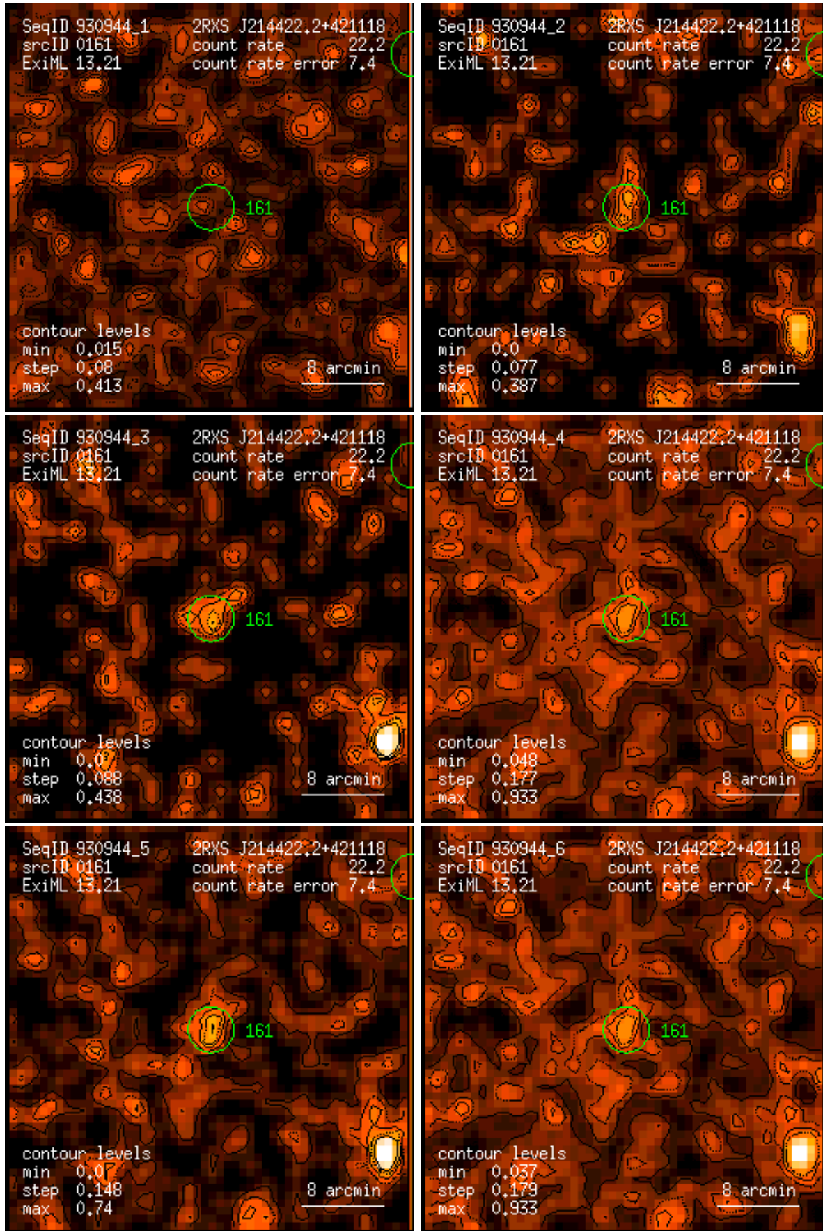
Figure 161: RASS 930944: detection 0161: band rate images, Gaussian filter: (1) PSPC channels 11 – 41, (2) 52 – 90, (3) 91 – 201, (4) 11 – 235, (5) 52 – 201, (6) 11 – 201. Broad band rates in counts/ks. Band rate contour levels in counts/ks/arcmin 2 .
