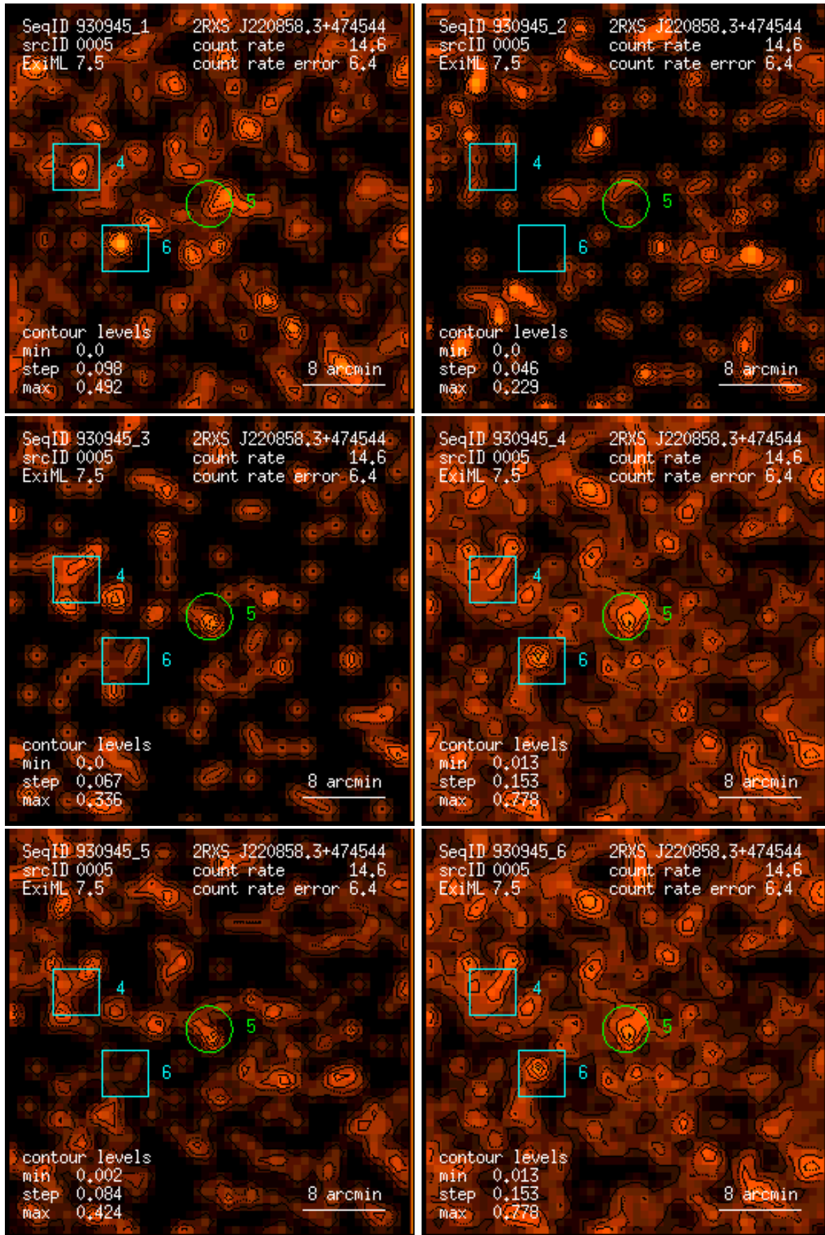
Figure 5: RASS 930945: detection 0005: band rate images, Gaussian filter: (1) PSPC channels 11 – 41, (2) 52 – 90, (3) 91 – 201, (4) 11 – 235, (5) 52 – 201, (6) 11 – 201. Broad band rates in counts/ks. Band rate contour levels in counts/ks/arcmin 2 .
