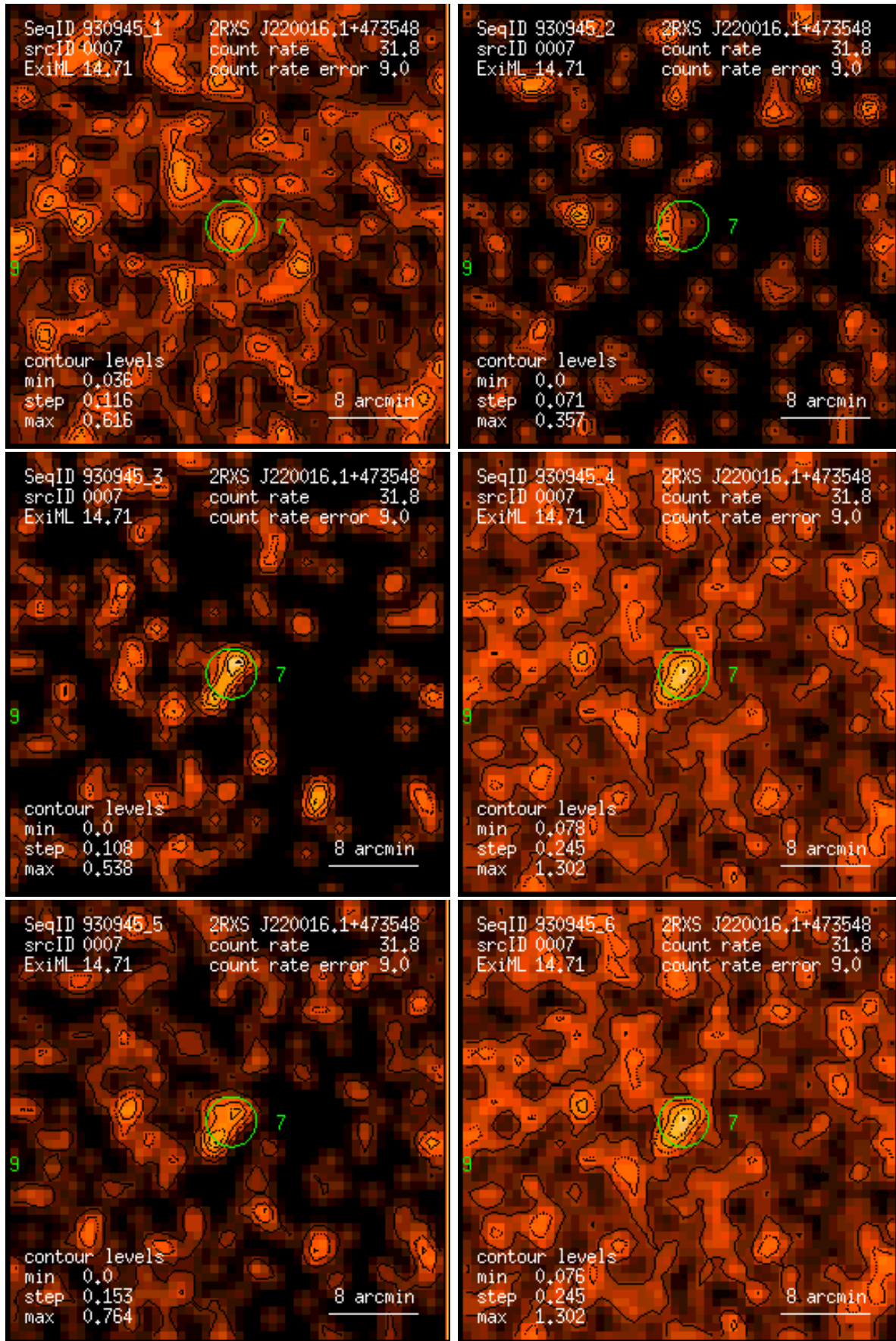
Figure 7: RASS 930945: detection 0007: band rate images, Gaussian filter: (1) PSPC channels 11 – 41, (2) 52 – 90, (3) 91 – 201, (4) 11 – 235, (5) 52 – 201, (6) 11 – 201. Broad band rates in counts/ks. Band rate contour levels in counts/ks/arcmin 2 .
