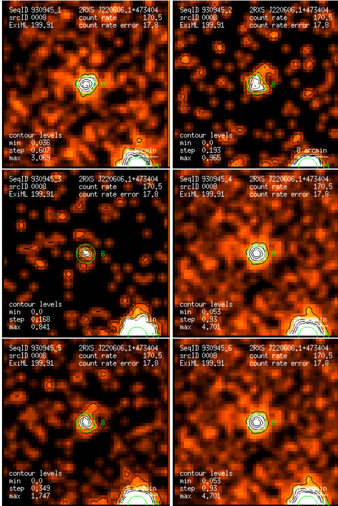
Figure 8: RASS 930945: detection 0008: band rate images, Gaussian filter: (1) PSPC channels 11 – 41, (2) 52 – 90, (3) 91 – 201, (4) 11 – 235, (5) 52 – 201, (6) 11 – 201. Broad band rates in counts/ks. Band rate contour levels in counts/ks/arcmin 2 .
