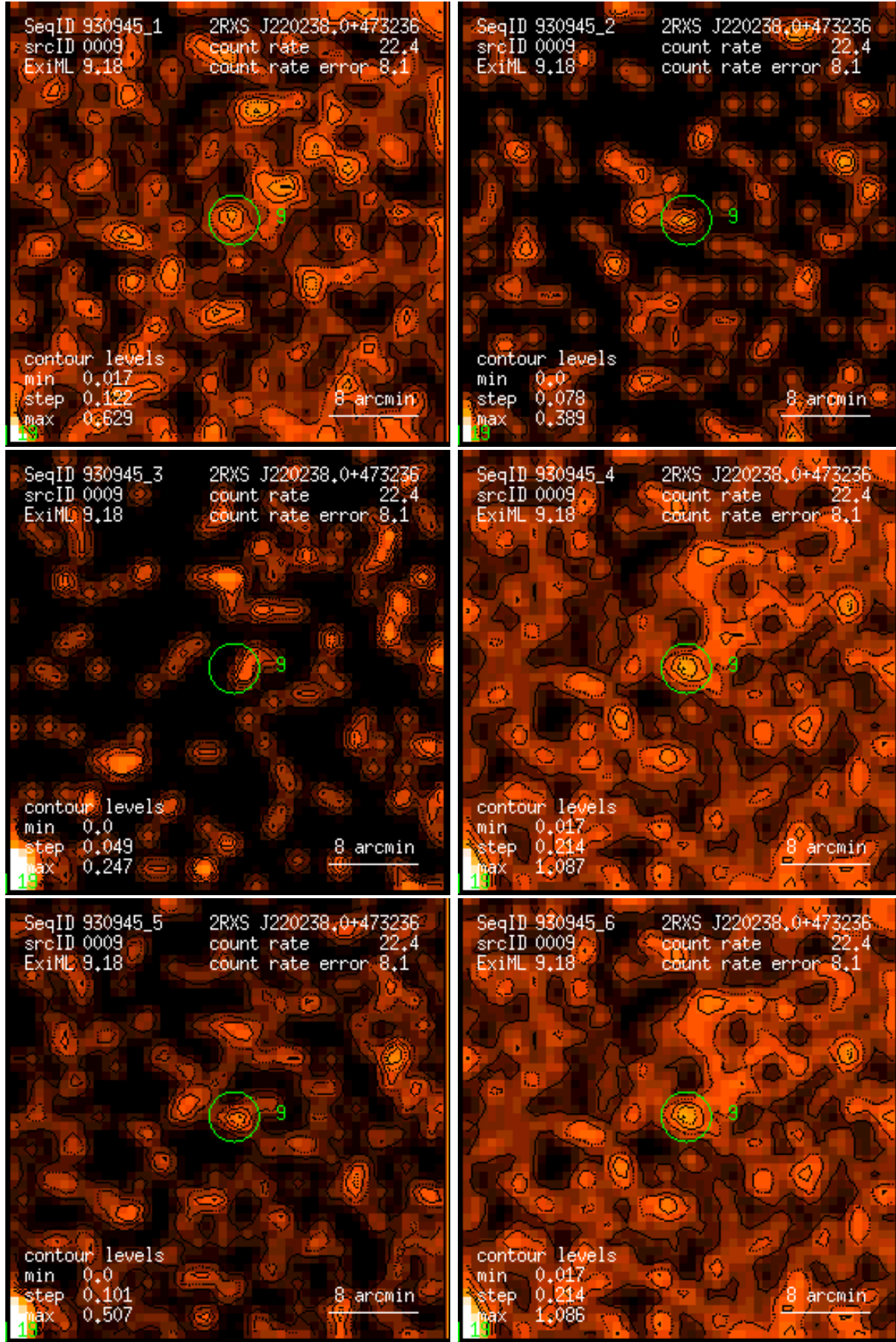
Figure 9: RASS 930945: detection 0009: band rate images, Gaussian filter: (1) PSPC channels 11 – 41, (2) 52 – 90, (3) 91 – 201, (4) 11 – 235, (5) 52 – 201, (6) 11 – 201. Broad band rates in counts/ks. Band rate contour levels in counts/ks/arcmin 2 .
