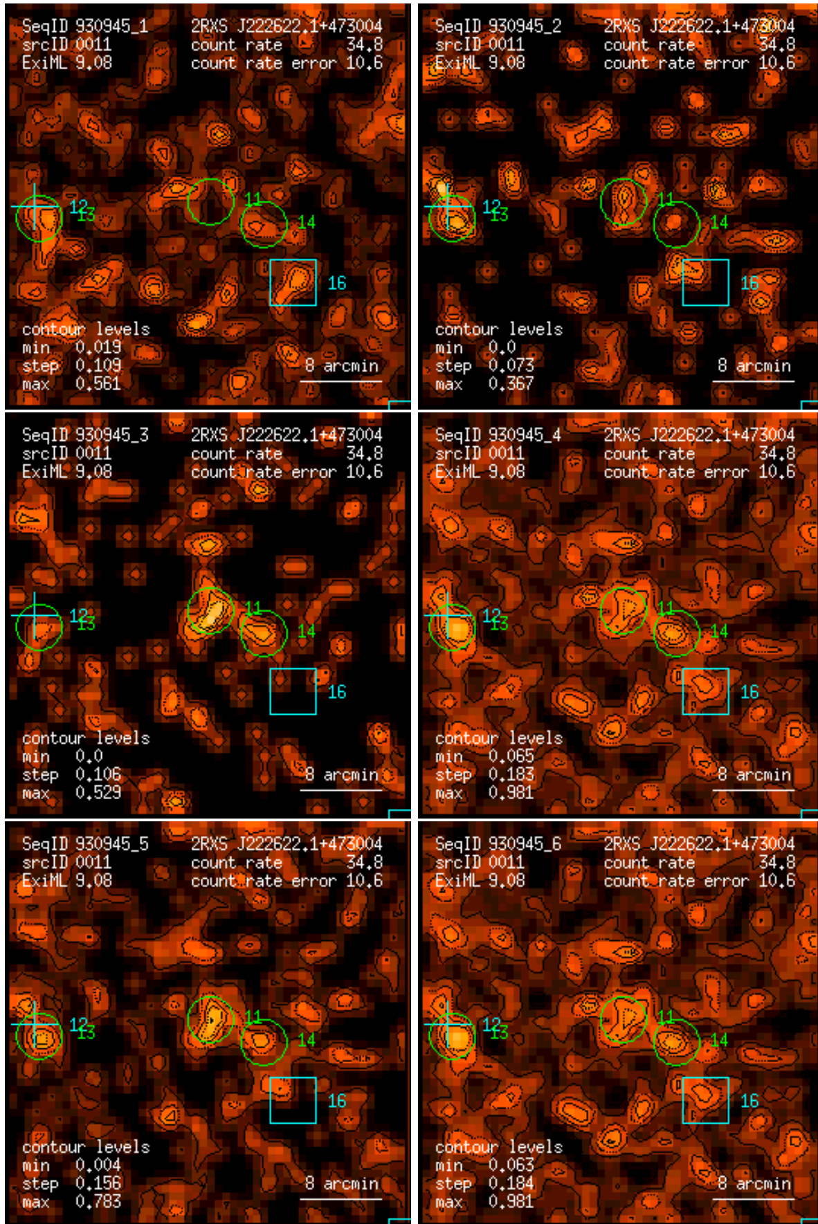
Figure 11: RASS 930945: detection 0011: band rate images, Gaussian filter: (1) PSPC channels 11 – 41, (2) 52 – 90, (3) 91 – 201, (4) 11 – 235, (5) 52 – 201, (6) 11 – 201. Broad band rates in counts/ks. Band rate contour levels in counts/ks/arcmin 2 .
